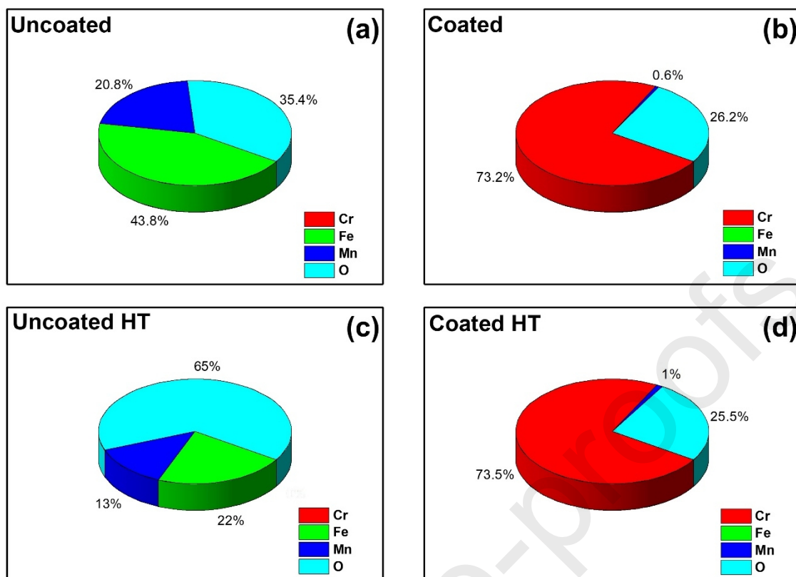
Figure 7 Atomic concentration of (a) uncoated, (b) Cr coated, (c) uncoated heat treated and (d) Cr coated heat treated SA508 powder calculated from HAXPES using Fe, Mn, Cr, O 1s.
