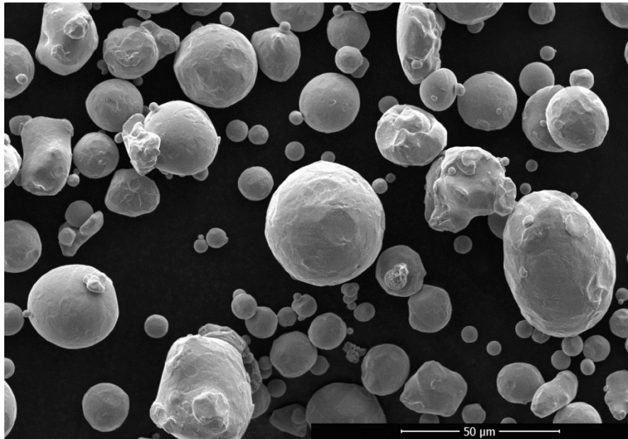
Figure 1 SEM SE image of gas atomized as-received SA508 low alloy steel powder
