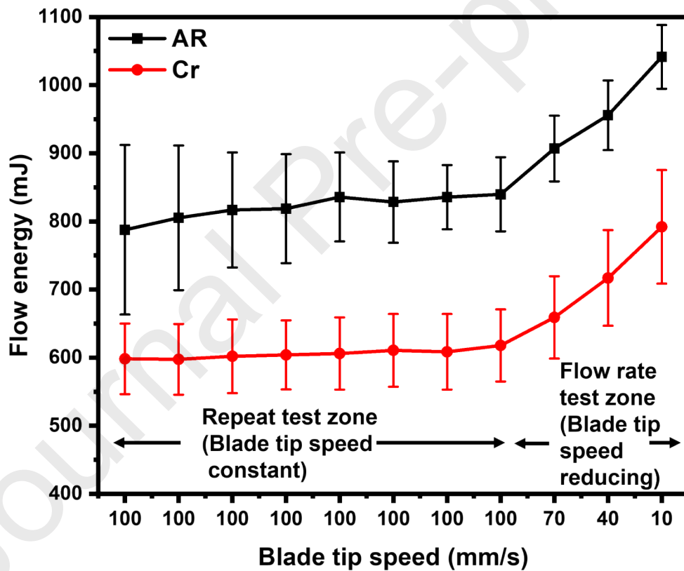
Figure 9 Downward flow energy of powder as a function of blade tip speed for uncoated and Cr coated SA508 powder. The standard deviation is measured from 3 tests
