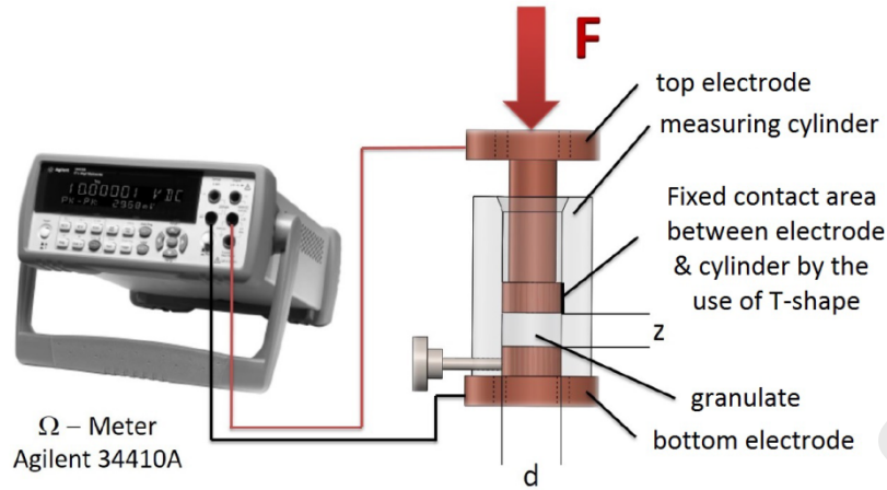
Figure 3 Schematic of equipment used to measure the electrical resistance of granular materials as a function of applied force [32].
