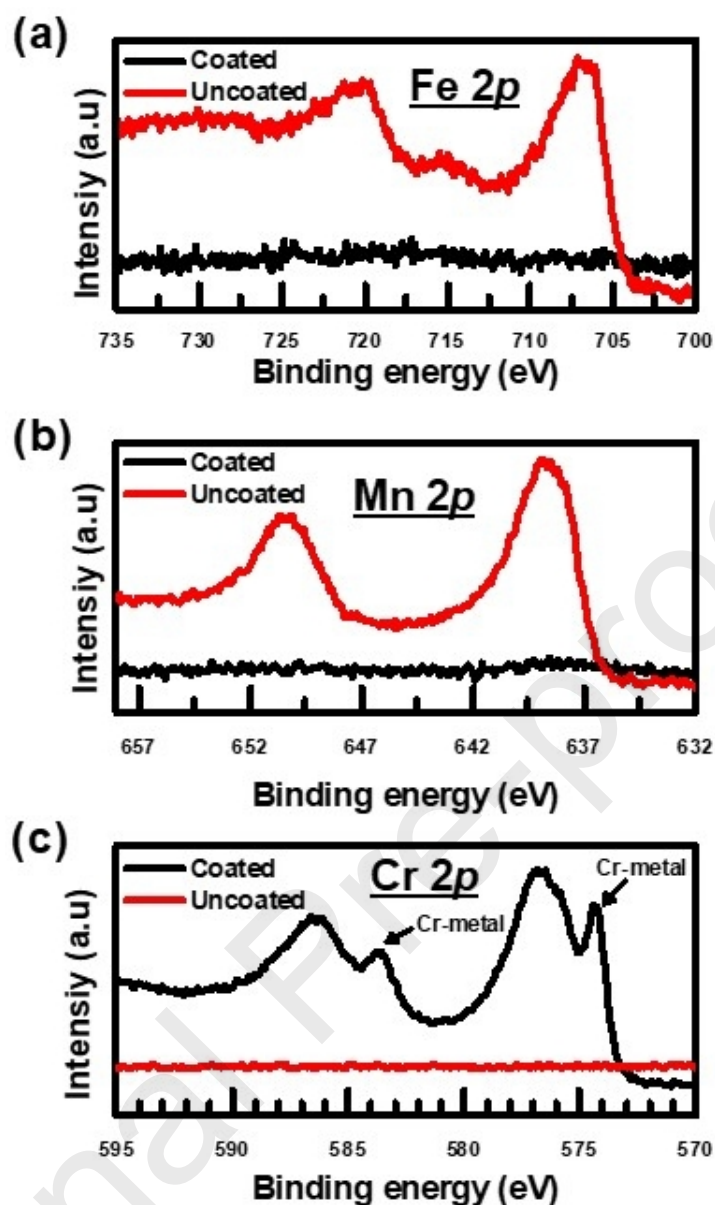
Figure 5 Core level XP spectra of (a) Fe 2p, (b) Mn 2p, and (c) Cr 2p, for an uncoated (red lines) and coated (black lines) samples.
