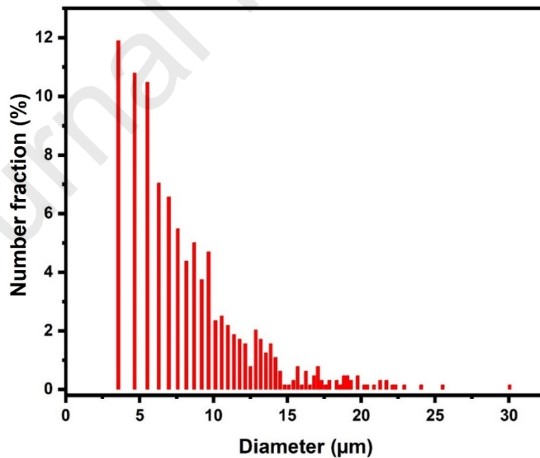
Figure 2 Particle size distribution of gas atomized as received SA508 low alloy steel powder. This was determined by taking a series of optical microscope images and using image processing software ImageJ [21] to estimate the mean diameter of individual particles. The distribution is reported without binning.
