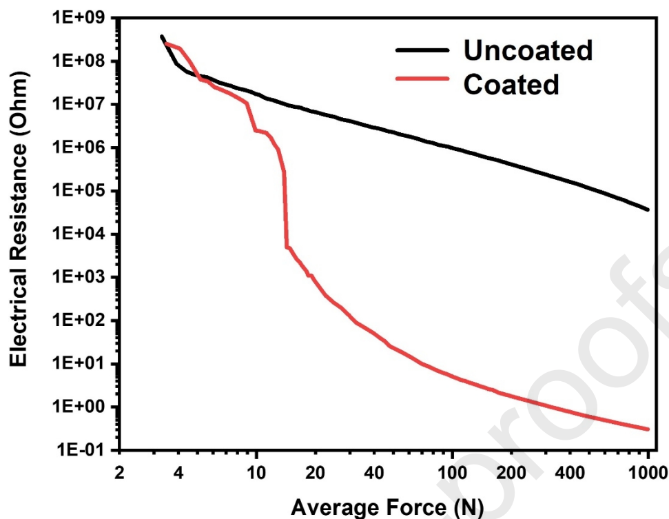
Figure 10 Mean electrical resistance of uncoated and Cr coated SA508 powder as a function of applied force.
