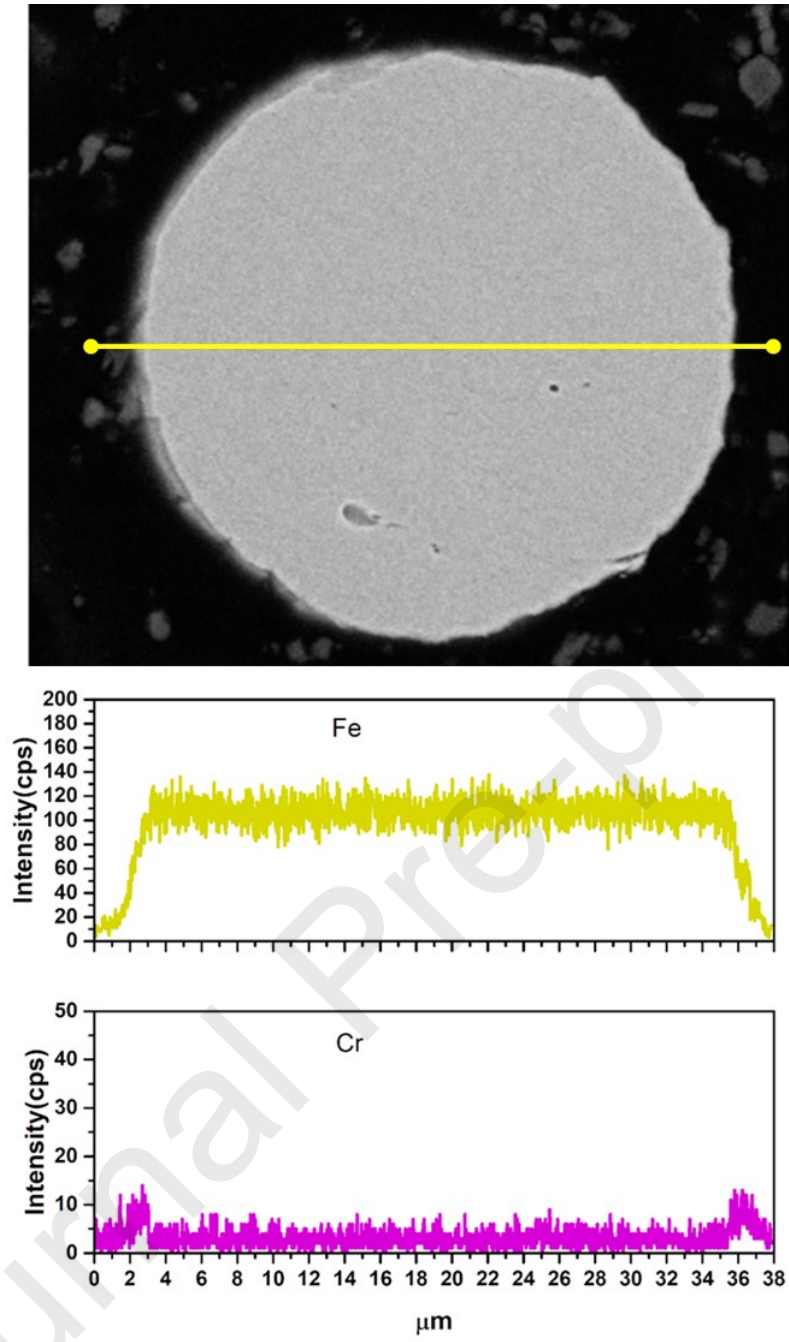
Figure 4 SEM SE Image of Cr coated powder particle and EDS line scans of Fe and Cr across a single powder
