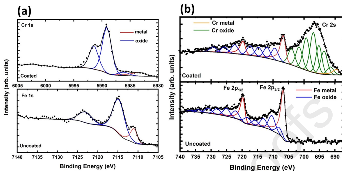
Figure 8 (a) Cr 1s and Fe 1s HAXPES spectra, and (b) Fe 2p / Cr 2s HAXPES spectra for Cr coated (top) and uncoated (bottom) SA508 powder. Metallic and oxide species have been peak fitted. Shirley backgrounds were used throughout.
