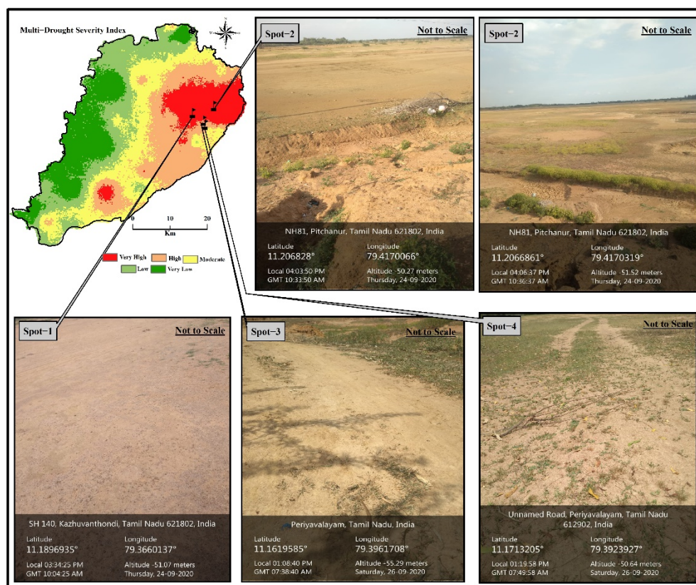
Figure 9. Multi-drought severity (i.e., meteorological, agricultural, hydrological), and field photographs of extreme-drought region (i.e., Jayankondam block), which implies that the region is exposed to extreme drought conditions.
