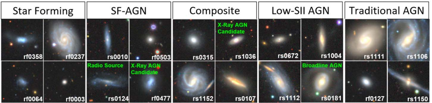
Figure 6. DECaLS DR8 images of representative RESOLVE galaxies in different categories of our optimized emission-line classification scheme (Section 3.2). Galaxies with nonoptical counterparts or previously cataloged broadline emission are labeled with green text.
