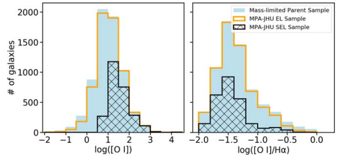
Figure 1. Distributions of [O I] line fluxes and [O I]/H\alpha ratios of the mass-limited parent, MPA-JHU emission-line (EL; H\alpha S/N > 5 ), and MPA-JHU SEL ( S/N > 5 for all SELs) samples in RESOLVE and ECO combined. The high S/N > 5 cut for the relatively weak [O I] line restricts our parent sample greatly but is required to use the emission line effectively.
