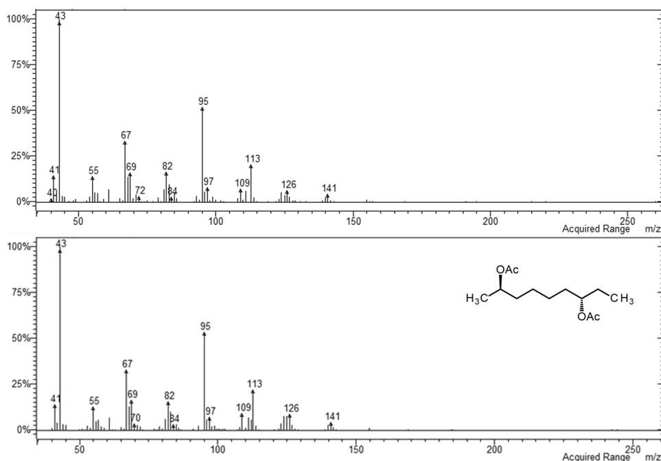
Fig. 4 Mass spectrum of major female-specific compound in volatiles from Contarinia brassicicola (upper) and synthetic (2 R ,7 S )-2,7-diacetoxynonane (lower)
