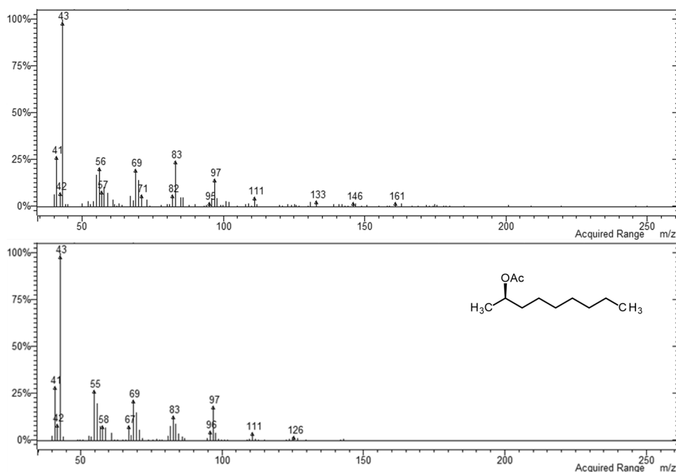
Fig. 5 Mass spectrum of minor female-specific compound in volatiles from Contarinia brassicicola (upper) and synthetic (2 R )-2-acetoxynonane (lower)
