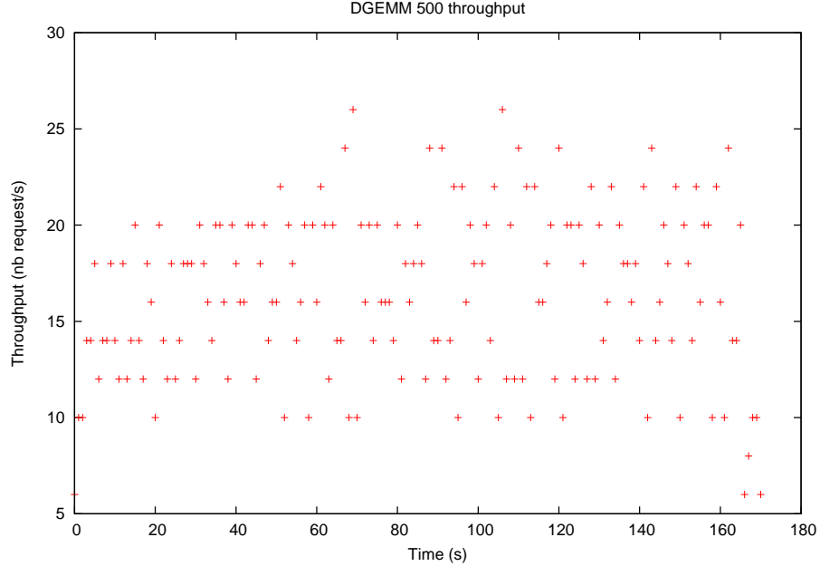
Figure 15: dgemm 500 throughput
