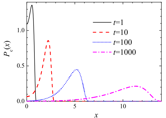
FIG. 19: (Color online): Evolution of the distribution P_c(x) with the time of stationary contact for the Lifshitz-Slözov coalescence mechanism ( \alpha = 1 and B = 1 ).
