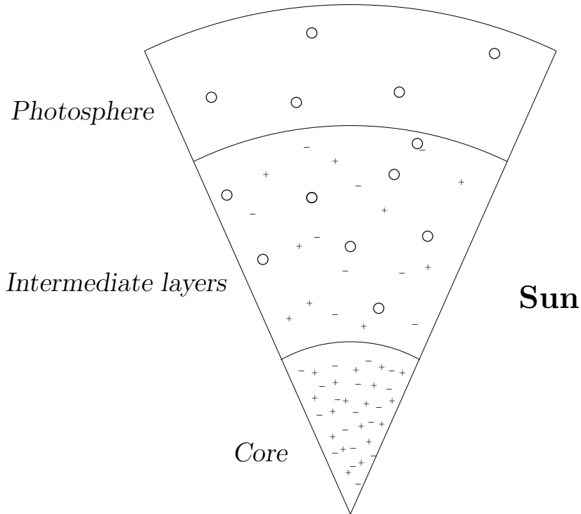
FIG. 2: A schematic view of the Sun. Signs + and – represent ionized protons and ionized electrons respectively, while circles represent hydrogen atoms.
