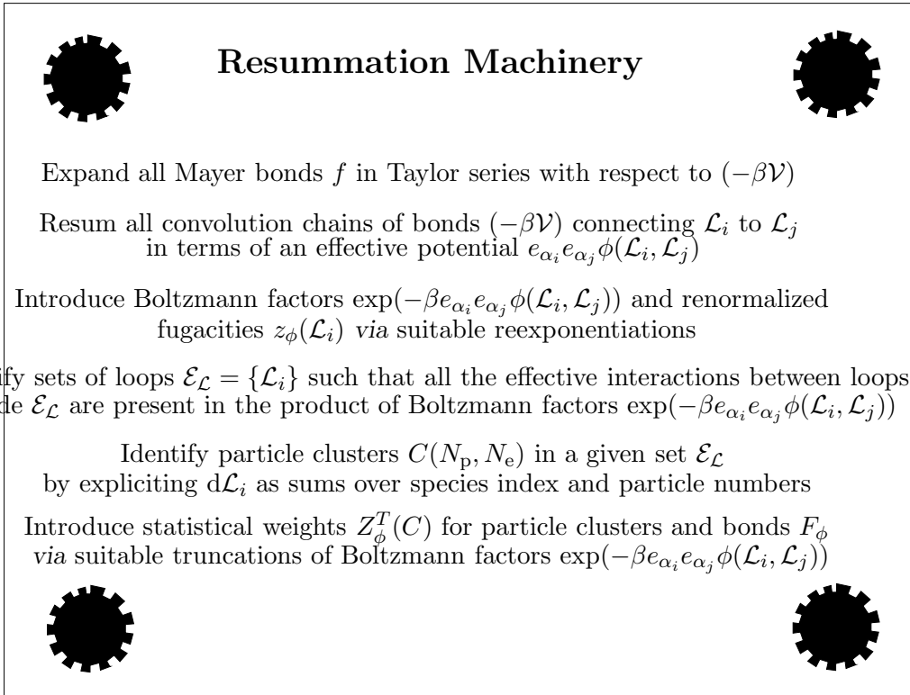
FIG. 7: Main steps of the resummation machinery.
