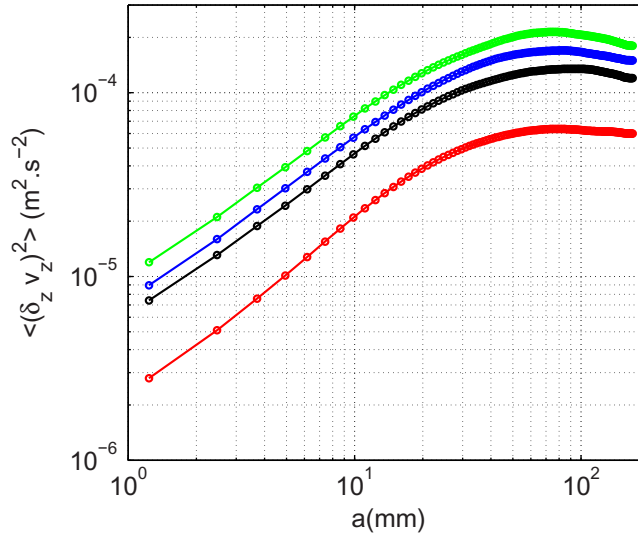
Figure 14. The second-order structure function \langle (\delta_z v_z)^2 \rangle of vertical velocity differences, for the various P values: red, P = 17.3 W; black, P = 45.2 W; blue, P = 65.9 W; green, P = 77.9 W.
