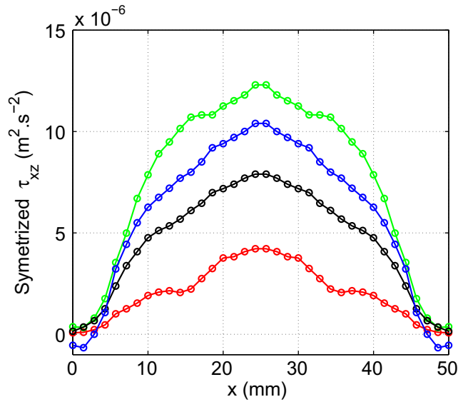
Figure 7. The transverse Reynolds \tau_{xz} stress for the four considered applied powers. Red, P = 17.3 W; black, P = 45.2 W; blue, P = 65.9 W; green, P = 77.9 W. These profiles have been symmetrized: (\tau_{xz}(x) + \tau_{xz}(d - x))/2 . Note its bell shape, while \tau_{zz} and \tau_{xx} were much flatter.
