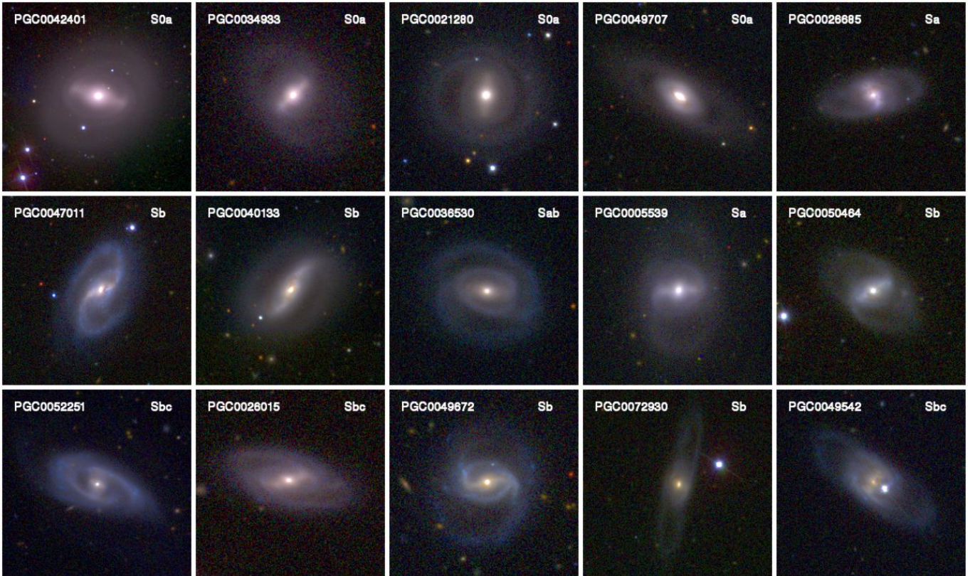
Fig. 16. Same as Fig. 3 for Pseudo-Ring attribute. As this is a low surface brightness feature, high-contrast pseudo-rings are preferentially shown here. The galaxies shown in the bottom row are the latest type galaxies (Sbc, Sb, Sb, Sbc resp.) with attributes values of 0.25, 0.5, 0.75, 1.0 respectively (for a fair comparison, an Sbc galaxy is also shown in the bottom row for attribute value 0).
