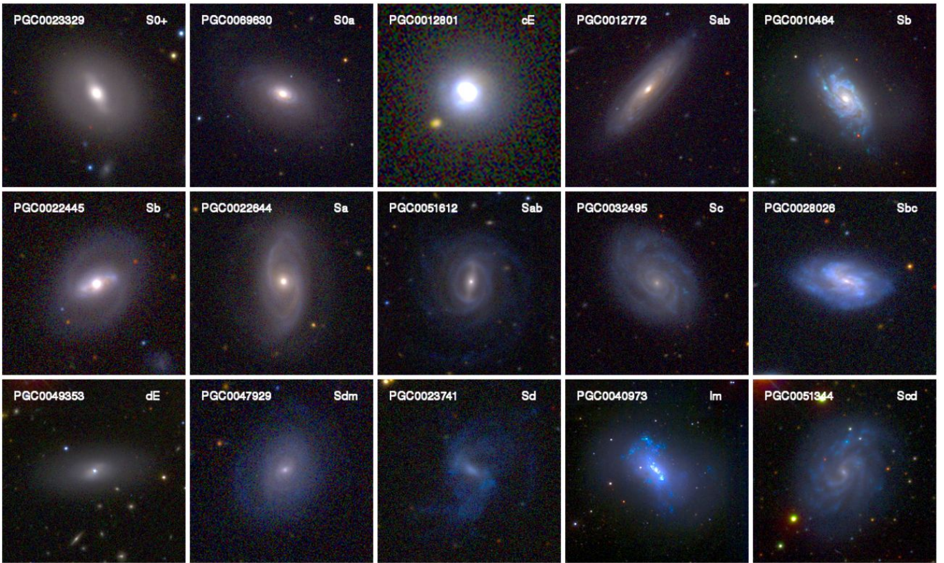
Fig. 13. Same as Fig. 3 for Flocculence attribute. Sab and Sb galaxies (PGC0012772 and PGC0010464) are shown in the top row because there are no earlier type galaxies with an attribute value of 0.75 or 1. We show in the left panel of the bottom row a nucleated dwarf lenticular galaxy classified as dE in the EFIGI catalogue, which has no flocculence; it however has an Hot Spot attribute value of 0.5 due to an unusually strong nucleus.
