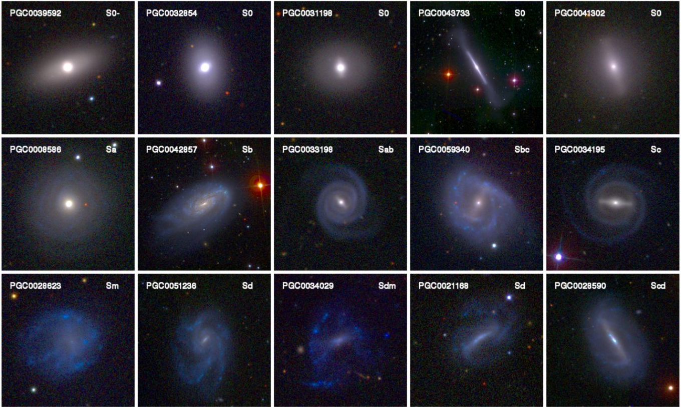
Fig. 15. Same as Fig. 3 for the Bar length attribute. Bar are frequent in all galaxy types except cE, cD, Ellipticals and dE. PGC0059340 (second panel from the right in the central row) illustrates that a bar can be long, hence a high attribute value of 0.75, but with a low surface brightness.
