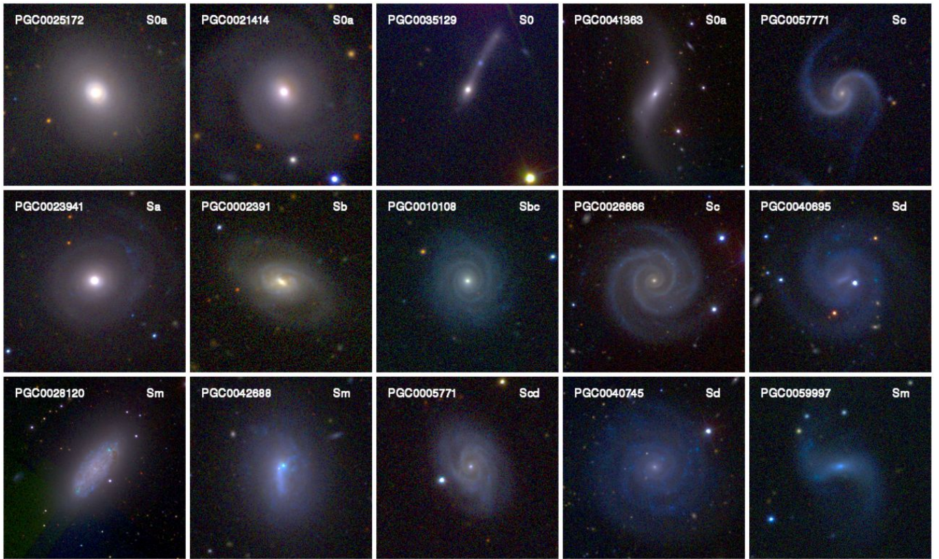
Fig. 9. Same as Fig. 3 for Arm strength attribute. Later types than announced in Fig. 3 are shown in the right panels of the top and central row because all earlier type galaxies have values less or equal to 0.75 for this attribute.
