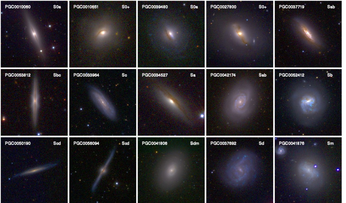
Fig. 12. Same as Fig. 3 for Dust dispersion attribute. PGC0037719 in the top right panel is the earliest type galaxy (Sab) with an attribute value of 1. The low values of the Dust dispersion attribute are preferentially seen in highly inclined galaxies, as indicated by the anti-correlation between both attributes in Fig. 20. Note the unusually faint bulge of Sab galaxy PGC0042174 (central row, second from the right).
