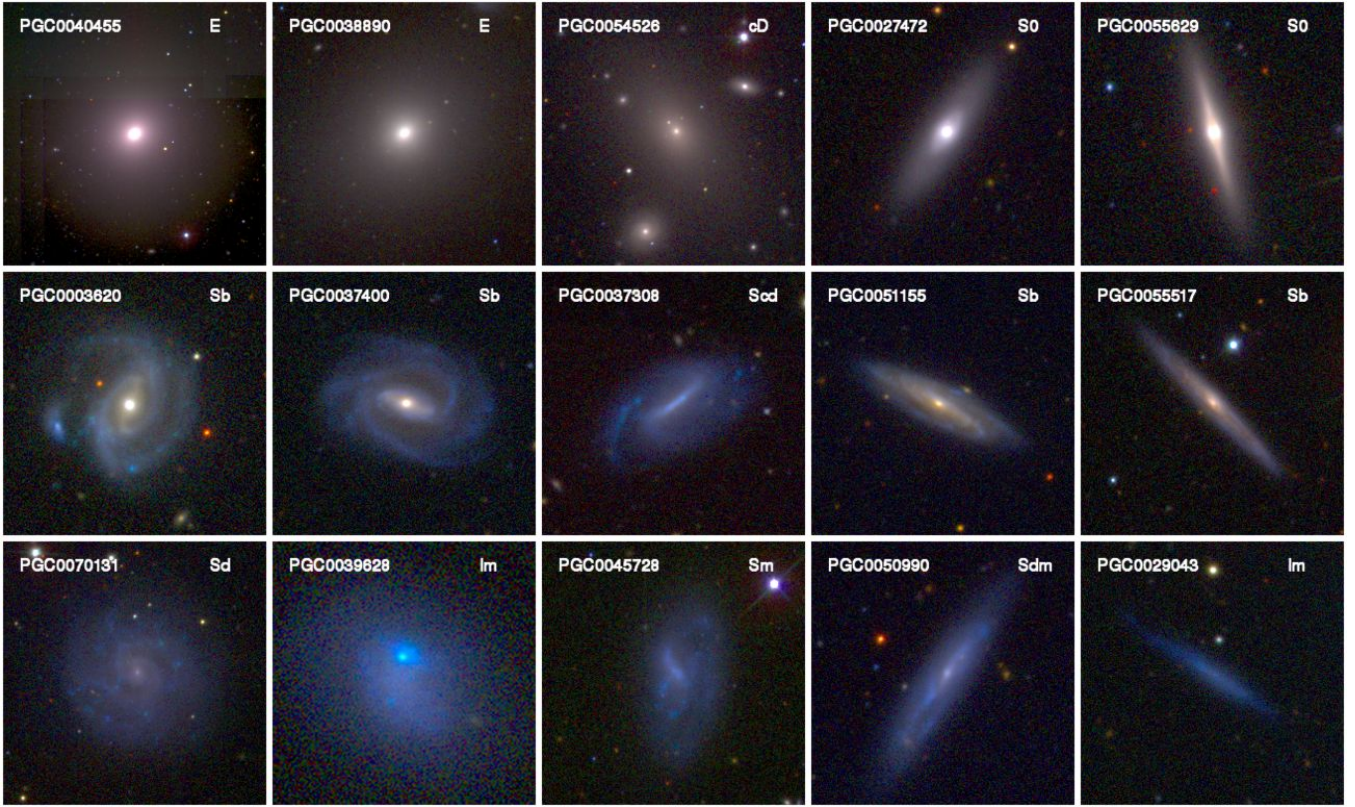
Fig. 3. Examples of EFIGI galaxies with the five possible values of the Inclination/Elongation attribute: 0 to 1 from left to right. The PGC number and the EFIGI Hubble type are indicated inside each image. For each attribute value, 3 types are shown: pure bulge (cE, cD, E), lenticular and S0a galaxies in the top row, early spirals in the middle row (from Sa to Scd), later spirals (Sd to Sm), Im and dE in the bottom row. Note the very low surface brightness of the Scd, Sd, Im and Sm galaxies in the central panel and the 2 left panels in the bottom row, typical of such objects which are numerous in the EFIGI catalogue. In all images, north is up and east to the left.
