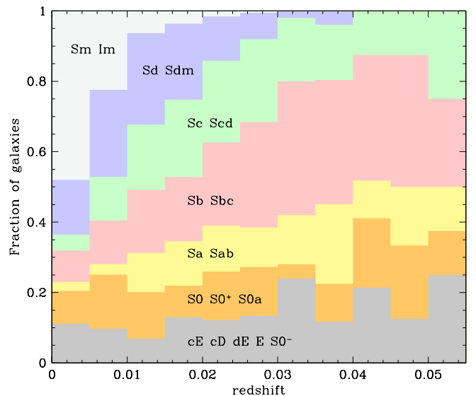
Fig. 27. Fraction of EFIGI galaxies with a given morphological type as a function of redshift.
