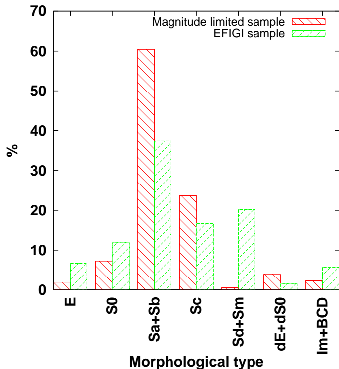
Fig. 29. Comparison between the observed EFIGI catalogue type mix (in green) and the expected type mix from a magnitude-limited sample with g < 15.75 (in red).
