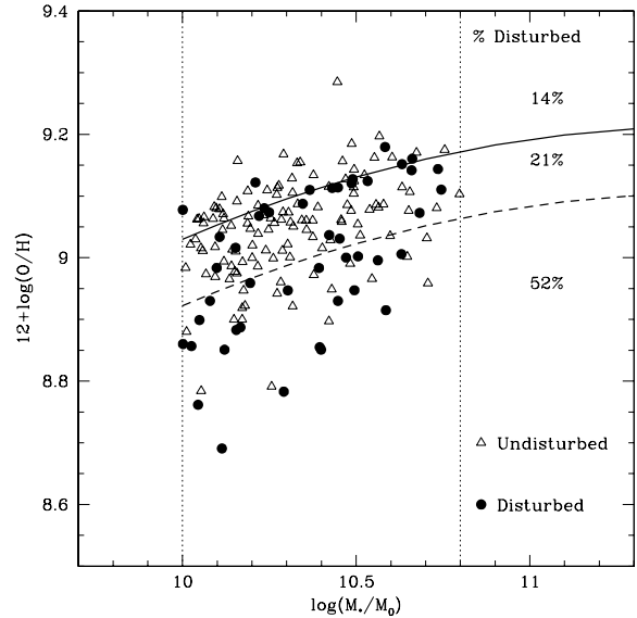
Fig. 5. Distribution of 12 + \log(\text{O}/\text{H}) and \log(M_*/M_\odot) values for galaxies with stellar masses in the range \log(M_*/M_\odot) \approx 10.0 to 10.8 . The circles correspond to disturbed galaxies and triangles to undisturbed galaxies. The solid and dashed lines indicate the limits of the high, medium, and low metallicity ranges. The solid line corresponds to the Tremonti et al. (2004) fit to the MZ relation shifted by +0.078 . The dashed line corresponds to this fit shifted by -0.03 dex.
