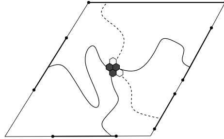
FIG 9. The landing sequences used to prove an upper bound on the probability of the 5-arm event. At most one site with five such arms exists.
