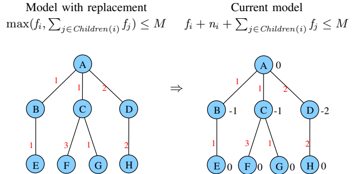
Figure 1. Transformation from the model with replacement.
