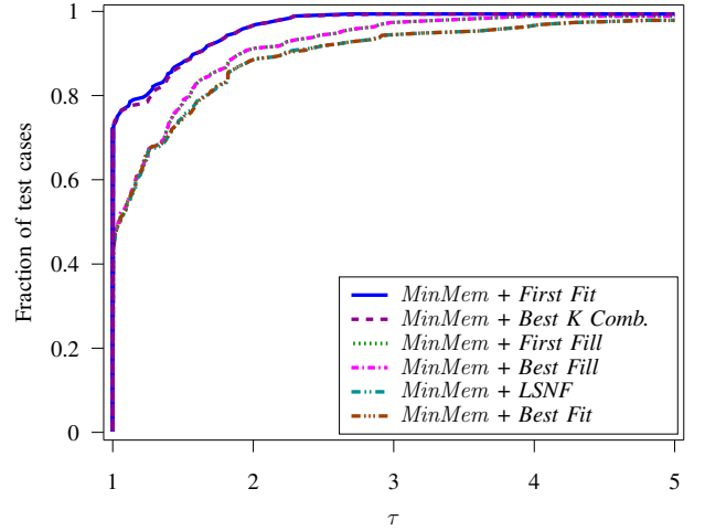
Figure 7. Performance profiles for comparing the resulting I/O volume of the heuristics for the MinMem algorithm on the assembly trees.
