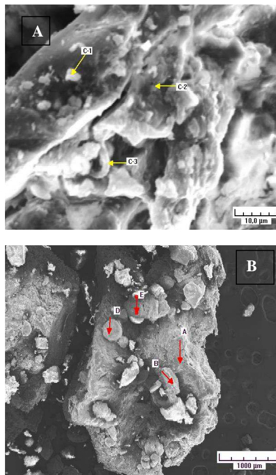
Figure 1. SEM image of sewage sludge (A: Urban Sludge and B: Industrial sludge)
