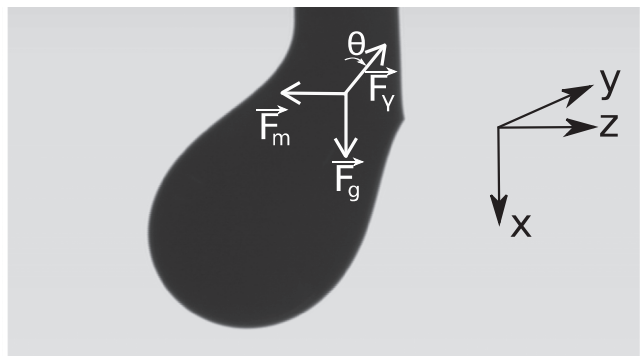
FIG. 3. Picture of a ferrofluid drop (APG) submitted to a magnetic force \vec{F}_m . \vec{F}_\gamma is the capillary force and \vec{F}_g is the gravity force.
