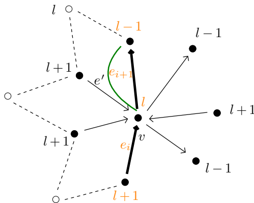
Figure 2: Two consecutive steps of a left-most geodesic.
