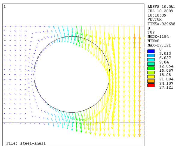
Fig. 7: Displacement vectors
