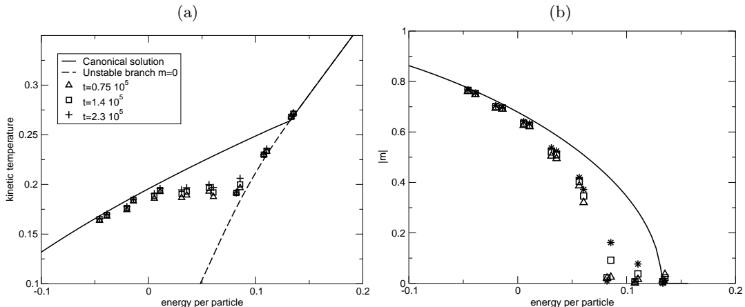
FIG. 5: Microcanonical results obtained using molecular dynamics simulations for the ferromagnetic \phi^4 model: \theta = 0.5 , N = 10^4 and water bag initial conditions q_0 = 1 , w_q = 10^{-4} .
