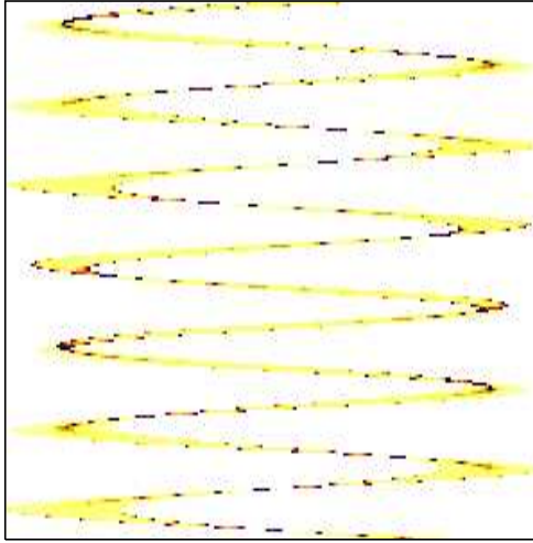
FIG. 1: Dynamics of the cluster. Evolution of the density \rho(q) of formula (5) in grey scale for short times. The darker the grey, the bigger the density. Space is horizontal, whereas the vertical downward direction corresponds to time. One notices the periodic motion with the characteristic time scale \omega_M^{-1} , defined in the text. In this simulation N = 4096 , \theta = 0.5 .
