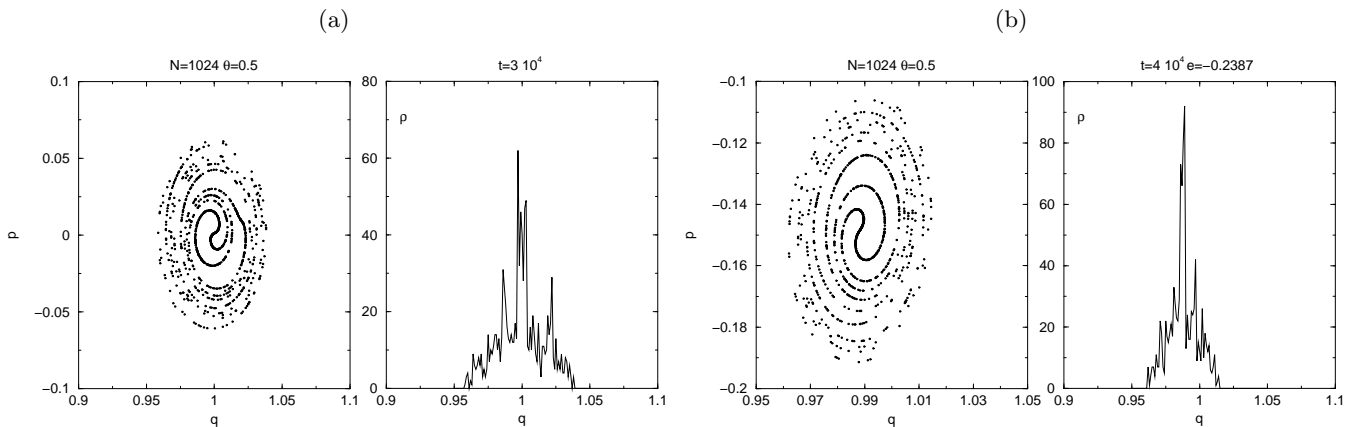
FIG. 2: Phase space snapshots of the cluster and the corresponding density \rho(q) of formula (5) at two different times. In this simulation N = 1024 , e = -0.2387 , \theta = 0.5
