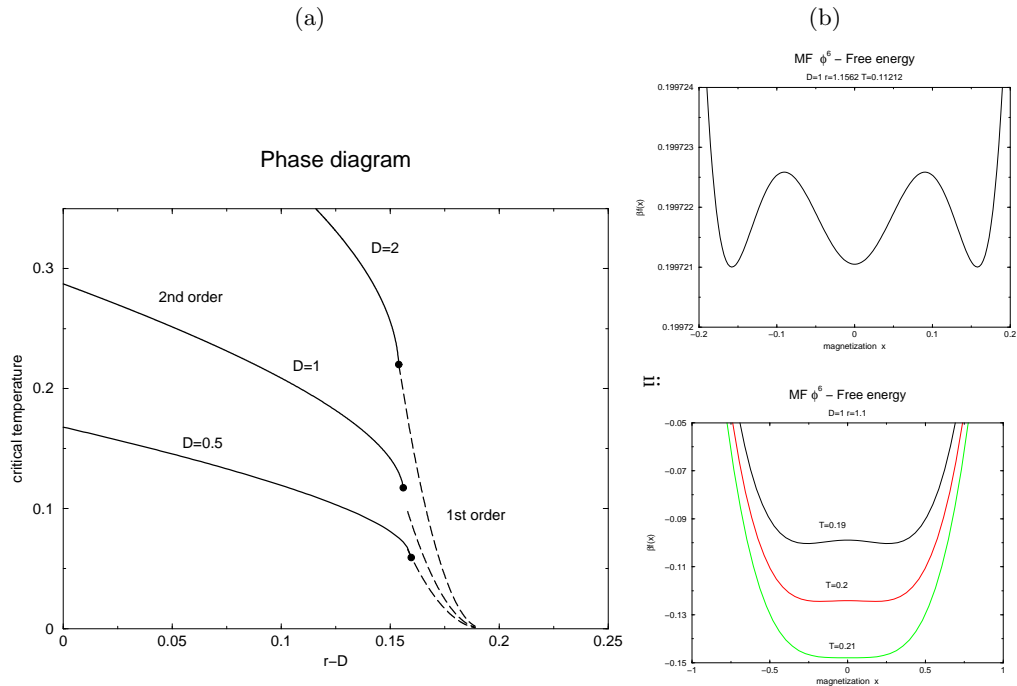
FIG. 6: Panel (a) shows the phase diagram of the \phi^6 model for different values of the coupling constant D . The solid (respectively dashed) line marks the second (resp. first) order critical line, and the full dots the tricritical points. Panels (b) present the Landau free energy at a first order transition close to the tricritical point T_{tr} and at a second order transition occurring on the line a = 0 , T_c = 0.205 .
