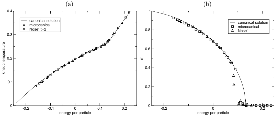
FIG. 4: Comparison of ensembles for the \phi^4 model, \theta = 0.5 , N = 512 : caloric (panel a) curve and magnetization (panel b). Squares and triangles refer to microcanonical and canonical simulations, respectively, while the solid lines are the exact canonical solutions given by Eqs. (25) and (24). The critical point is located at T_c = 0.264 ( e_C = 0.132 ). In both cases the initial conditions were q_i(0) = 1 and p_i(0) chosen randomly with a gaussian distribution.
