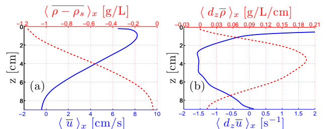
FIG. 2: (Color Online) The time averaged values of a) down-plane velocity \bar{u} (solid line, bottom axis) and density difference \overline{\Delta\rho} (dashed, top axis) and b) the vertical gradients d_z \bar{u} (solid, bottom axis) and d_z \bar{\rho} (dashed, top axis) as functions of the distance z from the plane. These profiles have also been averaged along the downstream distance ( \langle \bullet \rangle_x symbol), between 21 and 47 cm.
