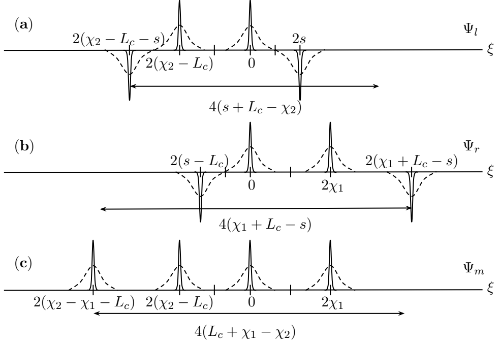
Figure 4.5: A schematic diagram showing the initial conditions (peaks in solid lines) for \Psi_l , \Psi_r and \Psi_m (from top to bottom), respectively. The dashed lines show the probability functions some time after t = 0 . The two-sided arrows indicate the period of each probability function.
