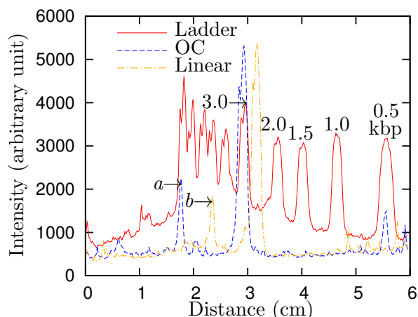
Figure 5.3: The profile of the fluorescence intensity of the stained DNA shown in Figure 5.2. The front of loading wells of the gel is designated as the origin of the distance. Here only the profiles of Lane A (ladder), F (open-circular pUC19) and G (linear pUC19) are displayed. The peaks indicated by a and b are the dimeric open-circular pUC19 and dimeric linear pUC19, respectively.
