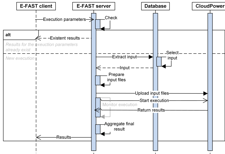
Fig. 3. General service execution flow.
