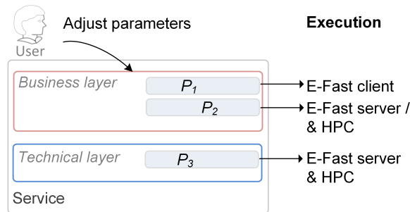
Fig. 4. Service general architecture.
