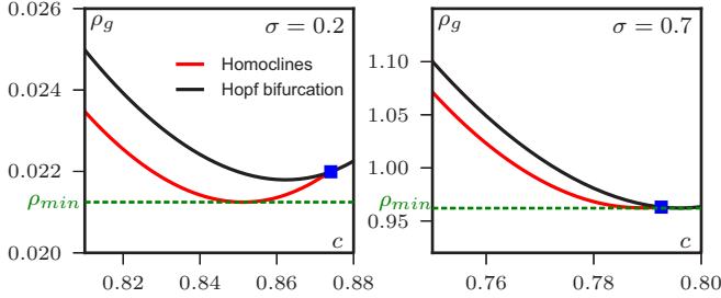
FIG. 18. (Color online) Propagative solutions of the Vicsek hydrodynamic equations for \sigma = 0.2 and 0.7 . The solution with the lower mean density \rho_{\min} is found at the minimum of the line of homoclinic solutions. At low noise, it does not coincide with the heteroclinic solution (blue squares). v_0 = 1 .
