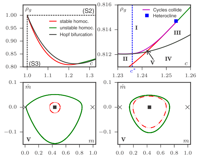
FIG. 20. (Color online) Top row: Phase diagram for the propagative solutions of Eq. (B4). The right plot is a zoom on the region c^* < c < c^h . Phases I to IV are the same as in the case a_4 = \text{cst} (see Fig. 6). Bottom row: Phase portraits of the solutions in phase V for the same c = 1.2421 and \rho_g = 0.81228 (left) and \rho_g = 0.81248 (right). When \rho_g increases, the size of the stable cycle decreases while the size of the unstable cycle increases, until they collide as indicated on the phase diagram. v_0 = \lambda = \xi = P_0 = \varphi_g = 1 .
