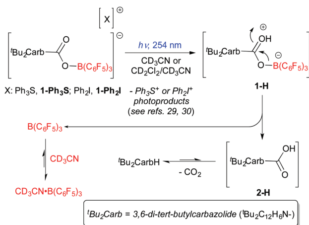
Scheme 2 Suggested mechanism for photorelease of B(C 6 F 5 ) 3 from 1-Ph 3 S .
