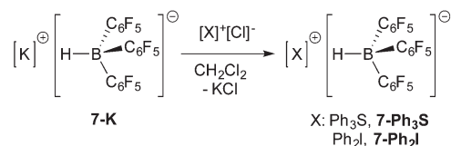
Scheme 4 Synthesis of hydridoborates 7-Ph 3 S and 7-Ph 2 I .
