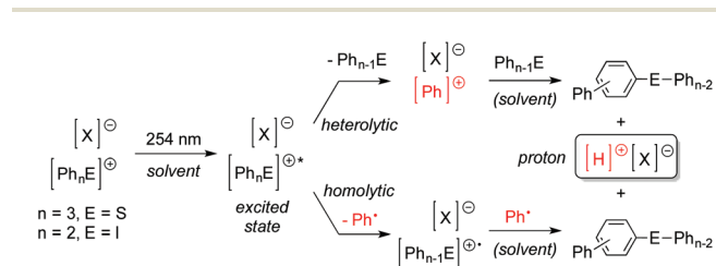
Scheme 5 Proton generation from photolysis of Ph n E cations.
