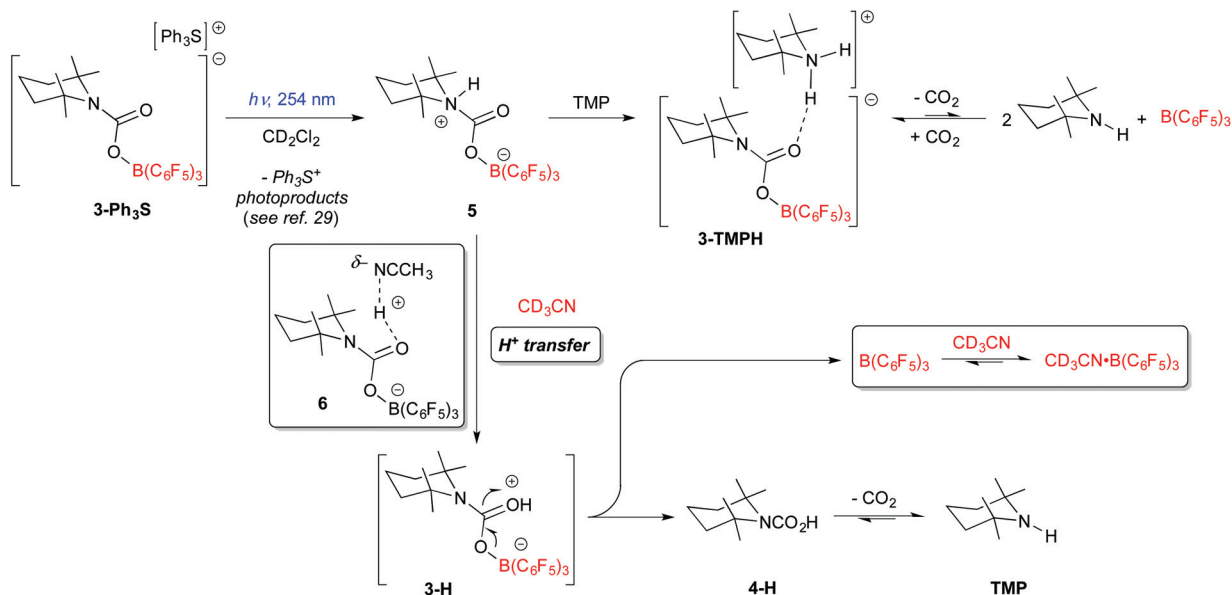
Scheme 3 Generation of 5 from 3-Ph 3 S under 254 nm light and suggested mechanism for photorelease of B(C_6F_5)_3 from 3-Ph 3 S in the presence of acetonitrile.
