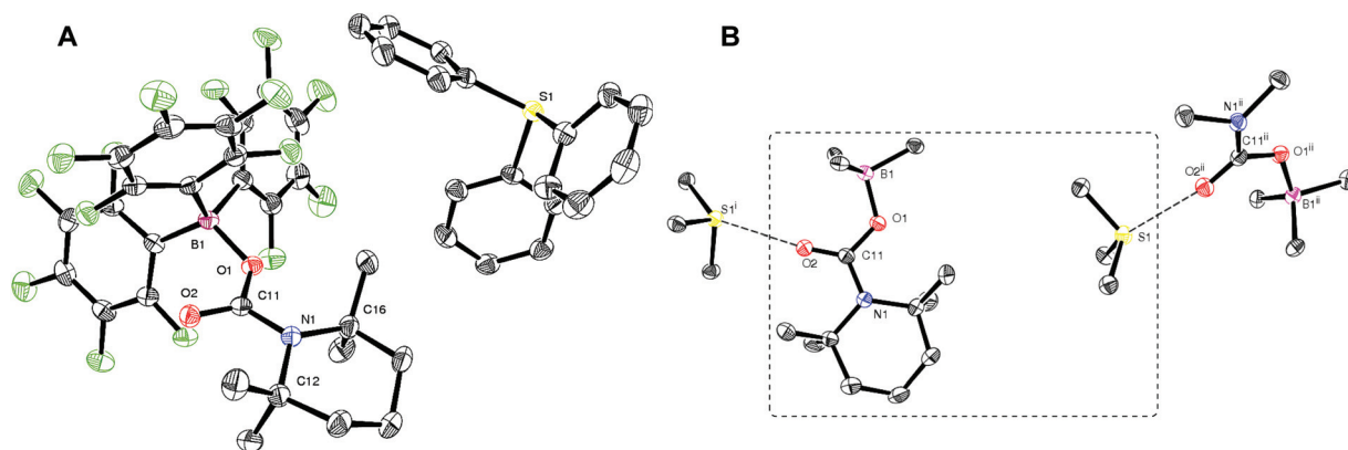
Fig. 1 (A) X-ray structure of 3-Ph 3 S (thermal ellipsoids drawn to 50% probability level). Hydrogen atoms are omitted for clarity. Selected bond distances (Å): B1–O1, 1.509(3); C11–O1, 1.328(3); C11–O2, 1.226(3); C11–N1, 1.386(3). Selected bond angles (°): B1–O1–C11, 120.96(19). (B) View showing C=O...S bonding motif in the unit cell of 3-Ph 3 S : S1 i ...O2 = S1...O2 ii , 3.025(2) Å.
