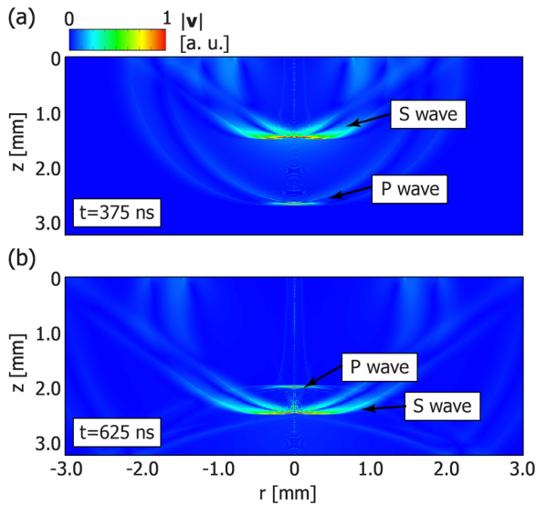
FIG. 11. Visualization of the wave field (magnitude of the velocity |v| ) in the far field at (a) 375 ns after the start of the 10 mJ pulse and (b) 625 ns after the start, by which time the still sharp P wave precursor has been reflected.
