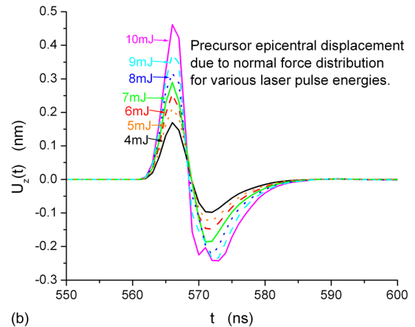
FIG. 8. Calculated epicentral displacement U_z^z(t) for a 3.12 mm thick tungsten plate resulting from the normal force distribution for (a) 10 mJ laser pulse energy, and (b) for a range of pulse energies on an expanded scale in the region of the P arrival.
