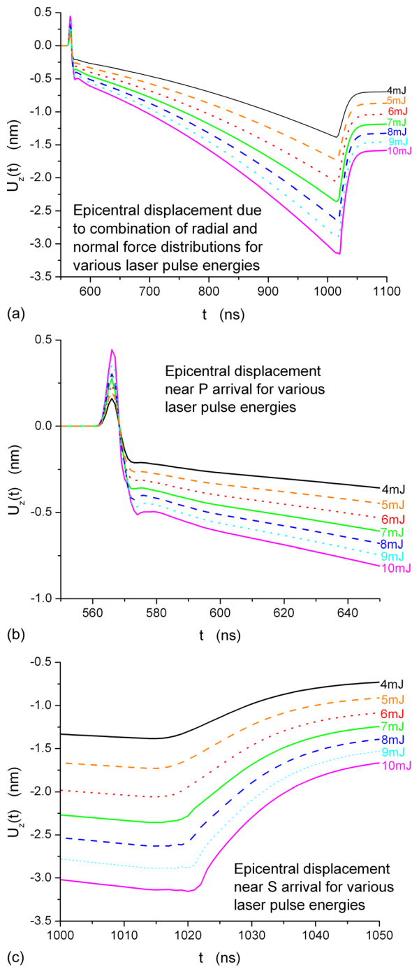
FIG. 9. (a) Combined epicentral displacement U_z^r(t) + U_z^n(t) for a range of laser pulse energies, (b) blup of region near P arrival and (c) blup of region near S arrival.
