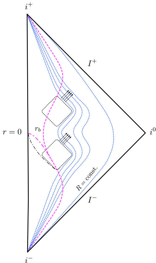
FIG. 2. Penrose diagram for the semiclassical radiation collapse model described by Eq. (7). The magenta thick-dashed line is the curve of the radius of the boundary of the collapsing object (the timeline defined by R_b(t) = r_b a(t) ), while the black thin-dashed lines represent the trapped surface. In the classical model, there is no bounce; at a certain time, the behavior departs from the semiclassical solution, as shown by the dotted-dashed lines (magenta thick line for r_b , black thin line for r_{ah} ). The blue-dotted lines are curves of constant radial coordinate.
