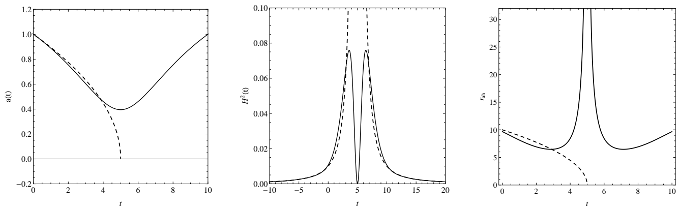
FIG. 3. Left panel: evolution of the scale factor a(t) for the classical radiation collapse (dashed curve) and the semiclassical radiation collapse (solid curve) in the case n = 2 . Central panel: as in the left panel for the square of the Hubble rate H^2 = (\dot{a}/a)^2 . Right panel: evolution of the radius of the apparent horizon r_{\text{ah}} for the classical radiation collapse (dashed curve) and semiclassical radiation collapse (solid curve). Here t_0 = 5 and \Lambda = 1
