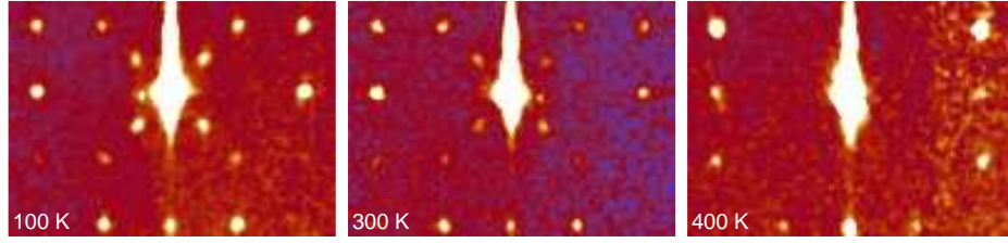
Figure 5.16: The (4,0,0) peak in the I4/mmm space group of AO/OO Y_{1-x}Sr_xCoO_{3-\delta} measured using single crystal X-ray diffraction at 400, 300 and 100 K. Additional peaks appear at positions corresponding to (3.5, 0.5, 0) and (3.75, 0.25, 0) as the crystal is cooled.
