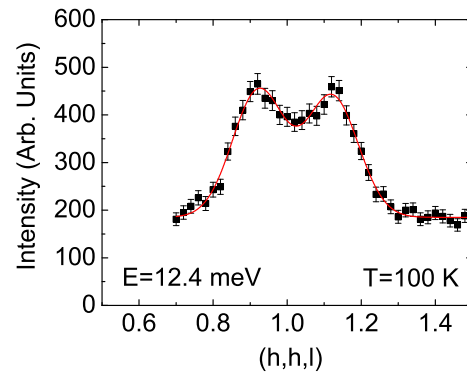
Figure 6.25: Scan along the (h, h, 2) direction across the (1, 1, 2) peak in the I4/mmm space group of Y_{0.15}Sr_{0.85}CoO_{3-\delta} measured at 100 K at an energy transfer of 12.4 meV on the the triple-axis spectrometer 2T1. The red line is the fit to the data.
