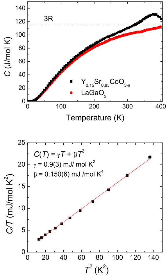
Figure 6.9: Upper panel: Temperature dependence of the specific heat of a single crystal of O 2 -annealed Y 0.15 Sr 0.85 CoO 3- \delta . LaGaO 3 , a non-magnetic perovskite, was also measured and is shown to indicate the lattice contribution to the recorded signal. The horizontal line indicates the value of 3R per atom for Y 0.15 Sr 0.85 CoO 3- \delta . Lower panel: C/T vs T^2 for the low temperature specific heat ( 2 < T < 10 K) of a single crystal of O 2 -annealed Y 0.15 Sr 0.85 CoO 3- \delta . The fit is to a model consisting of the electronic ( \gamma T ) and the lattice ( \beta T^3 ) contributions to the specific heat, which appears to be a good description of this low temperature data.
