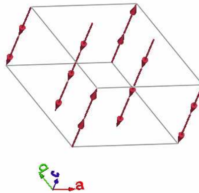
Figure 8.4: SDW and CAFM magnetic unit cells and the positions of the cobalt atoms in the structural unit cell. The top left panel shows the positions of the nonmagnetic Co1 (blue) and magnetic Co2 (red) cobalt atoms in the \text{Ca}_3\text{Co}_2\text{O}_6 unit cell. The PDA magnetic structure of the SDW phase is shown in the top right panel and the bottom panel shows the CAFM magnetic phase.
