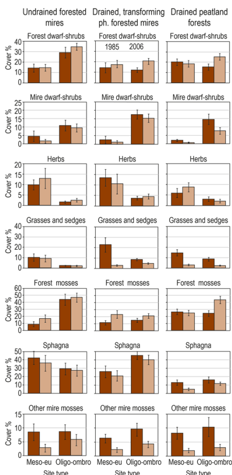
Fig. 2. The mean percentage covers (+ s.t.e.m.) of the functional species groups of vegetation according to two site fertility levels and three drainage phases in 1985 and 2006.
