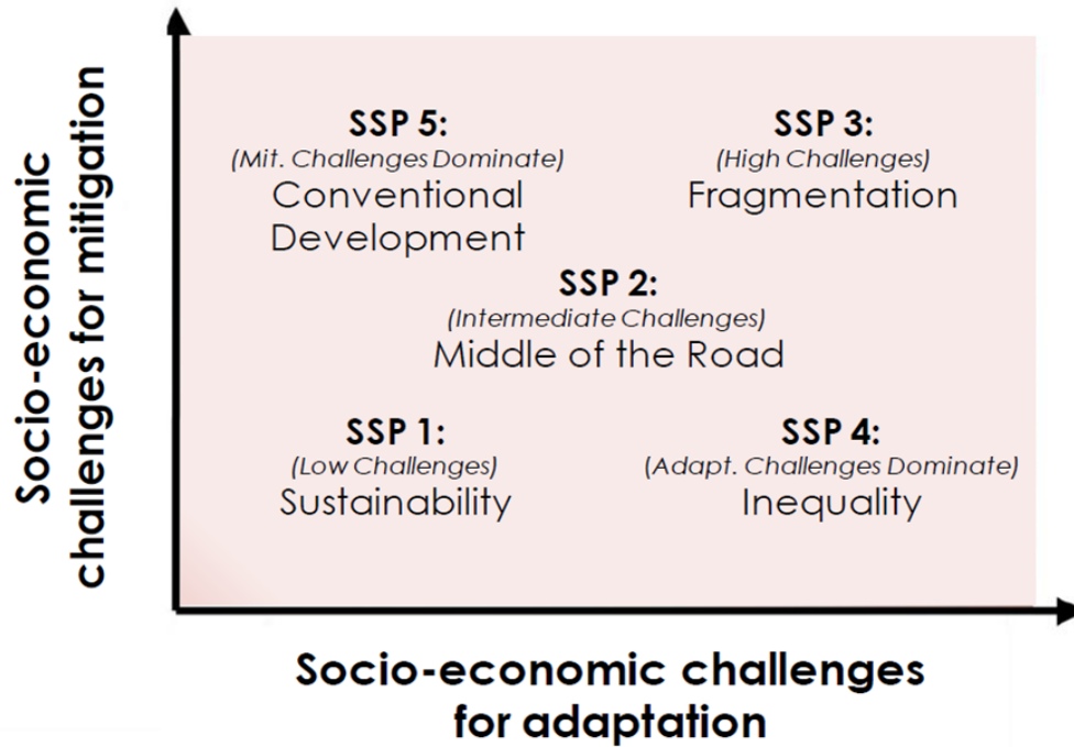
Figure 2: Socioeconomic Pathways.
