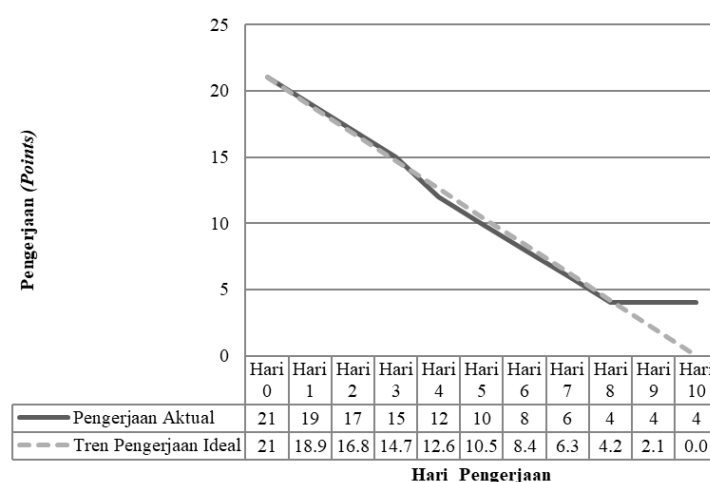
Gambar 4 Burn down chart sprint 2.
