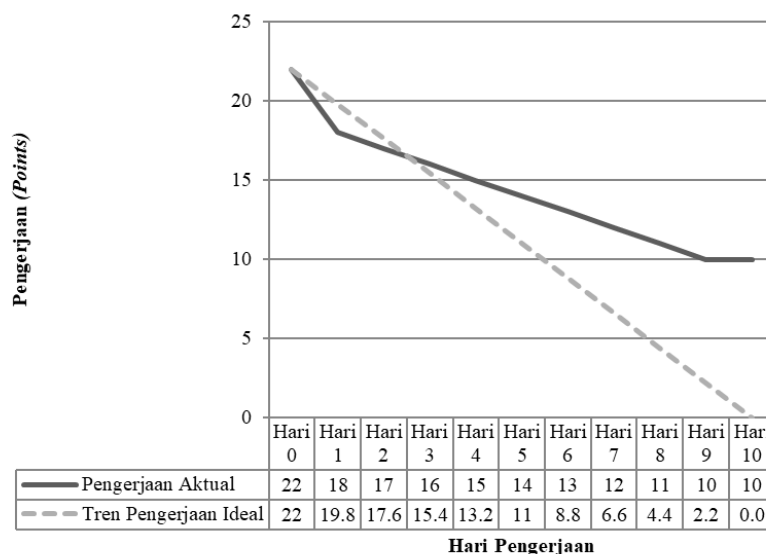
Gambar 3. Burn down chart sprint 1.
