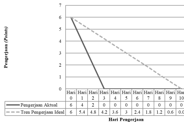
Gambar 17 Burn down chart sprint 4.
