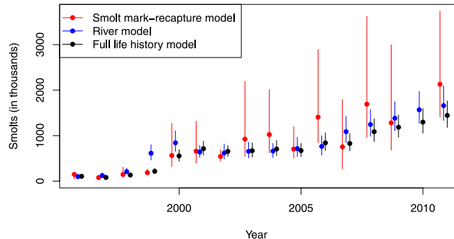
FIG. 3. The estimate of smolt abundance in the Tornionjoki River after sequential modeling steps B, C and the life-history model shown in Figure 2.
