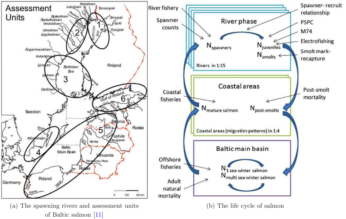
FIG. 1. The Baltic sea and the life cycle of salmon.
