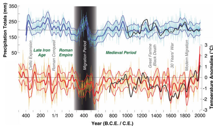
Fig. 3.1 Reconstructed April–June (AMJ) precipitation totals ( top ) and summer (June–August) temperature anomalies ( bottom ) for central Europe with respect to 1901–2000. Error bars are \pm 1 RMSE (Root-Mean Square Error) for the calibration periods. Black lines show independent precipitation and temperature reconstructions from
