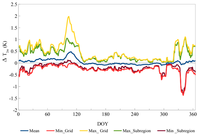
Figure 6. Maximum, minimum and mean differences of grid pointwise and regionally averaged 11-day running mean of daily mean 2 m air temperature over 15 years in subregion1.
