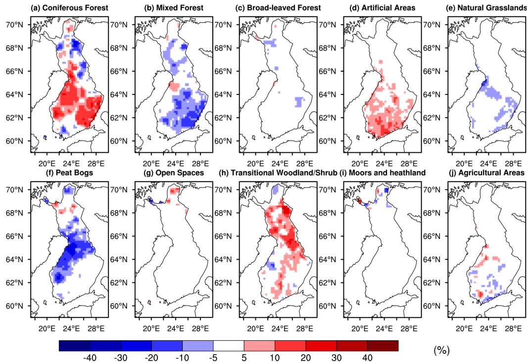
Figure 2. Changes of fractional coverage of the 10 land cover classes in Finland from the 1920s to the 2000s (FNFI10–FNFI11).
