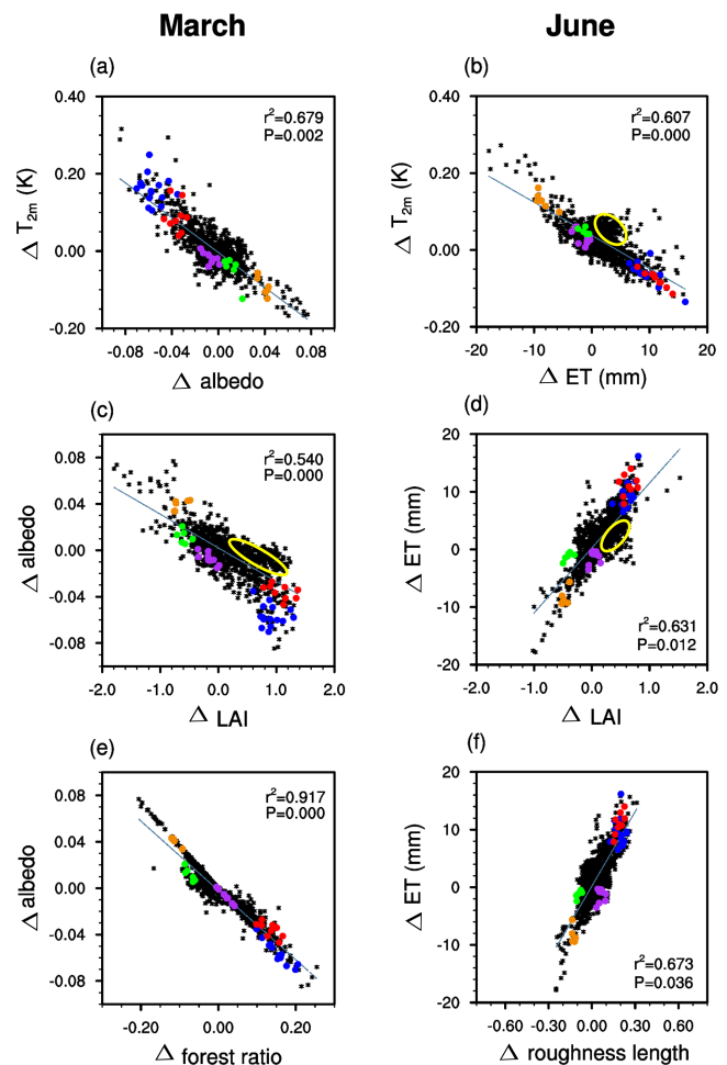
Figure 8. Spatial correlations between (a) changes in monthly-averaged daily mean 2 m air temperature ( T_{2m} ) and changes in albedo for March, (b) changes in T_{2m} and changes in ET for June and relationships between changes in land surface parameters in REMO LSS following land cover changes and changes in albedo (c, e) (changes in ET, d, f) in the corresponding month. The changes in the grid boxes in selected subregions are shown with coloured dots (subregion1 – blue; subregion2 – red; subregion3 – purple; subregion4 – green; subregion5 – orange). The grid boxes in yellow circles show the changes in the southeast area of Finland.
