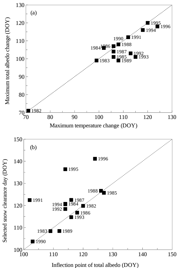
Figure 7. (a) Correlation between maximum temperature change day (DOY) and maximum total albedo change day (DOY); (b) correlation between inflection day of total albedo (the day when surface albedo just finishes a fast decrease from its wintertime level; DOY) and the snow clearance day (DOY). The plots show regional means over subregion1 for all 15 years.
