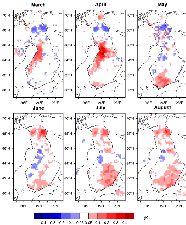
Figure 3. The 15-year averaged differences (FNFI10–FNFI1) in monthly-averaged daily mean 2 m air temperature in spring and summer months.
