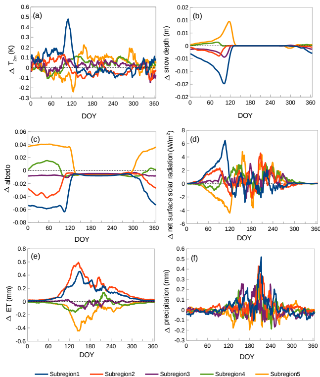
Figure 5. The 15-year averaged regional mean differences (FNFI10 – FNFI1) in 11-day running mean of daily mean (a) 2 m air temperature, (b) snow depth (presented as equivalent water), (c) surface albedo, (d) net surface solar radiation, (e) ET and (f) precipitation of the five subregions.
