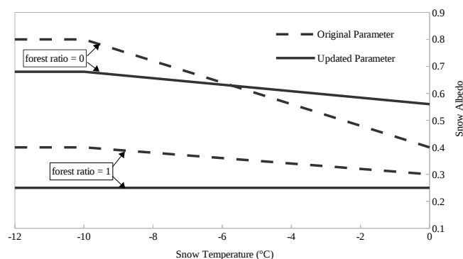
Figure B1. Modified snow albedo values in the snow albedo scheme (modified based on Fig. 3.6 in Kotlarski, 2007).
