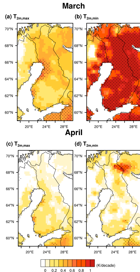
Figure 9. Temperature trends over 40 years (1959–1998) for (a, c) monthly mean daily maximum and (b, d) monthly mean daily minimum surface temperatures of March and April. The areas covered with black dots are statistical significant ( p < 0.1 ).
