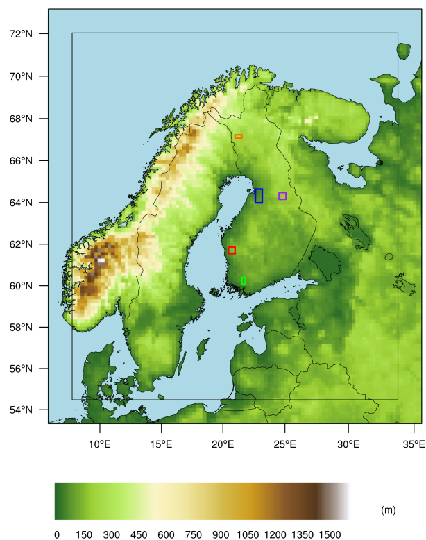
Figure 1. Orography of the model domain and the five selected subregions (subregion1 – blue; subregion2 – red; subregion3 – purple; subregion4 – green; subregion5 – orange). The inner black frame shows the extent of the relaxation zone from the outer boundary, i.e. the eight outer-most grid boxes in each direction of the model domain.
