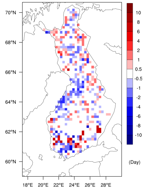
Figure 4. The 15-year averaged differences (FNFI10–FNFI1) in the snow clearance days over model grid boxes in Finland.
