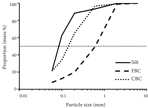
Fig. 1. Particle size for the studied media components expressed as the percentage passing sieve sizes; horizontal line denotes the 50% proportion
