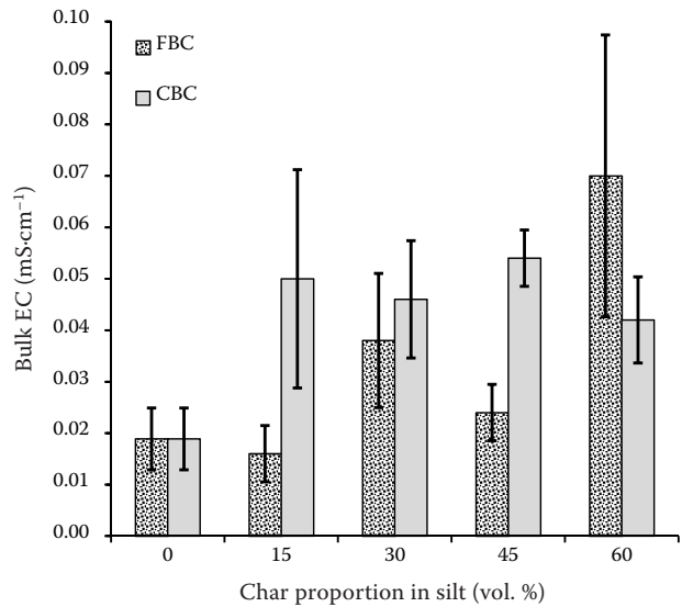
Fig. 3. Average electrical conductivity in the different growing media during the experiment (mean \pm SD)
