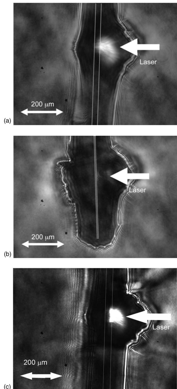
FIG. 2. (a) Shadowgraph of 25 \mu\text{m SiO}_2 + 1 \mu\text{m Cu} back layer taken at t_0 + 200 ps. (b) Shadowgraph of 4 \mu\text{m Al}/1 \mu\text{m Ni}/1 \mu\text{m CH} taken at t_0 + 200 ps. The dotted lines mark the position of the original target surfaces. (c) An example of 25 \mu\text{m CH} + 1 \mu\text{m Cu} back layer taken at t_0 + 200 ps.
