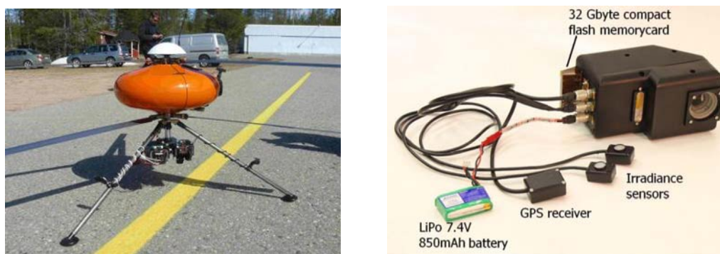
Figure 1. Infotron IT-180 UAV helicopter with both the CIR camera and Hyperspectral imager payload and flight configuration of UASI 2012 hyperspectral Imager.
