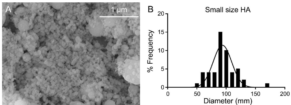
Supplementary Figure S2. SEM image and size distribution of hydroxyapatite nanoparticles (nHAPs). (A) SEM image shows the size of nHAPs adopted to fabricate CHAS. (B) The size distribution of nHAPs obtained from the SEM image was fitted to a Gaussian function. The diameter of nHAPs are using ImageJ software (V1.8.0_172, NIH, USA) ( https://imagej.nih.gov/ij/ ).
