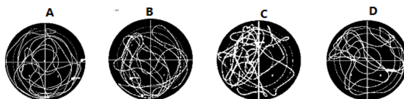
Fig 3: Tracings of the typical swim patterns in the probe trials (trial 21) at the control (A), captopril5 (B), 10 (C), 15 (D) mg/Kg group tested. The escape platform was on North West quadrant.
