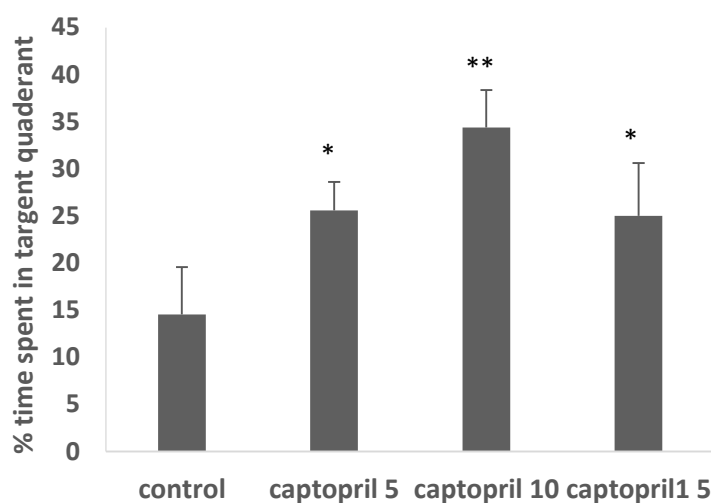
Fig 2: Water maze Mean ( \pm SEM) percentage of time spent in target quadrant. Morris water maze during probe trials. Asterisks indicate a significant difference from control (* P < 0.05 ; ** P < 0.01 ).
