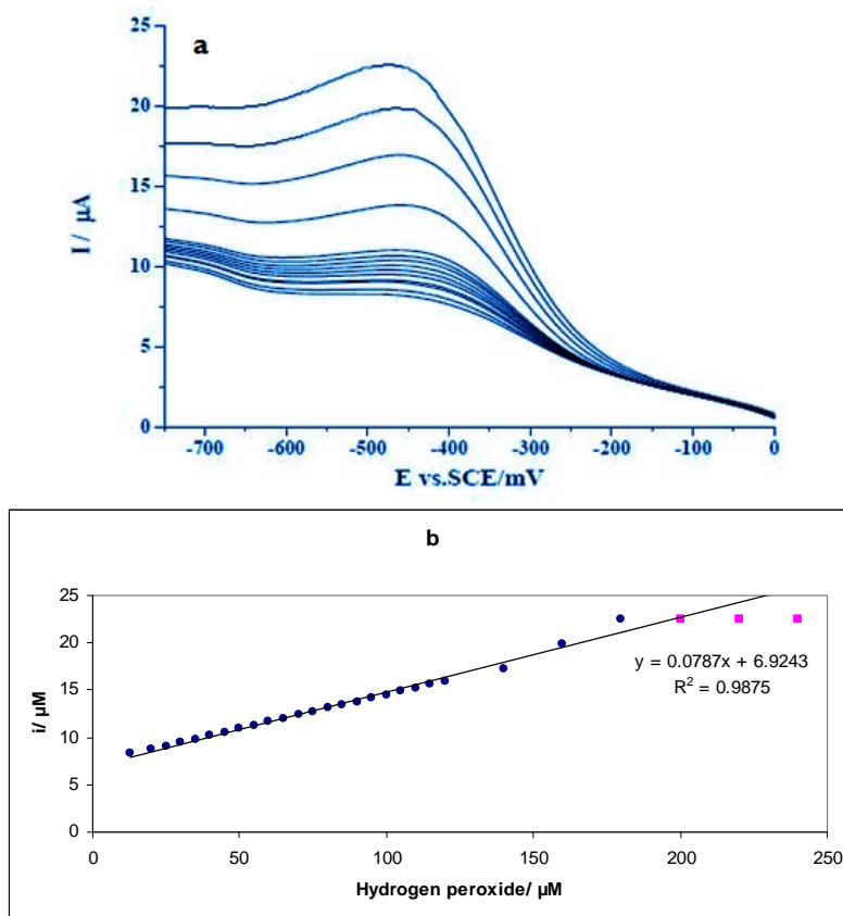
Fig. 7: (a) Cyclic voltammograms obtained at an Hb/ Zn Nps/ CPE electrode in 0.1M phosphate buffer solution (pH 7.0) for different concentrations of hydrogen peroxide and (b) the relationship between cathodic peak current of Hb and different concentrations of hydrogen peroxide (scan rate: 50 mVs -1 ).
