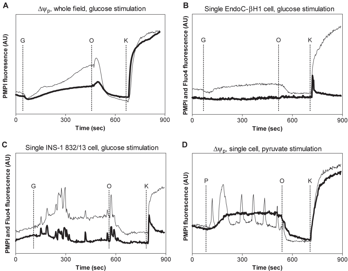
Fig 5. Plasma membrane potential and cytoplasmic free Ca^{2+} changes in EndoC-βH1 and INS-1 832/13 cells. Whole-field plasma membrane potential changes (A) in EndoC-βH1 (bold line) and INS-1 832/13 (thin line) cells. Additions: G, glucose, 16.7 mM; O, oligomycin, 0.5 ng/μL; K, KCl, 25 mM. Plasma membrane potential (thin line) and the free cytoplasmic Ca^{2+} (bold line) in (B) a single EndoC-βH1 cell and (C) a single INS-1 832/13 cell. (D) Representative single cell plasma membrane potential changes in response to pyruvate stimulation (P, 10 mM) in EndoC-βH1 (bold line) and INS-1 832/13 (thin line) cells. Data shown are representative for n = 3 experiments.
