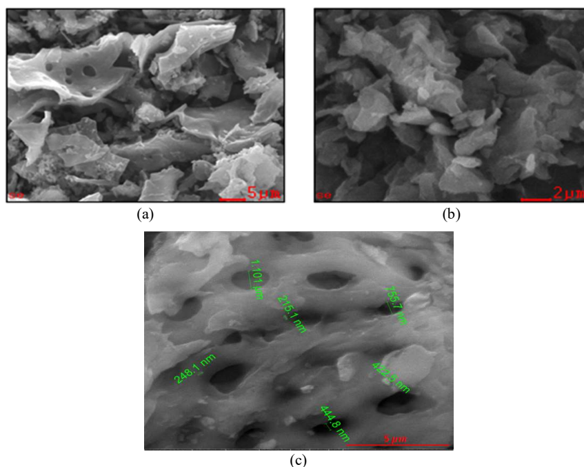
Figure 1 SEM images of (a) corncob powder, (b) RGO powder, and (c) RGO-PEG powder.
