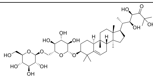
Goyaglycoside-h
