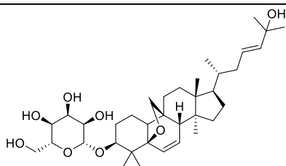
Momordicoside F2
