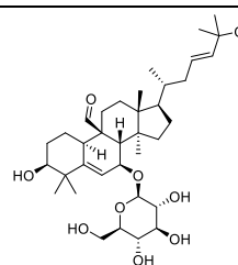
Momordicoside K
