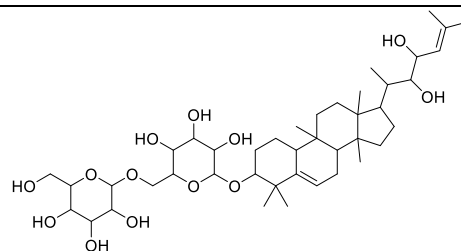
Momordicoside D
