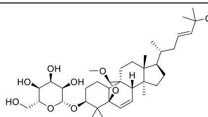
Goyaglycoside-d
