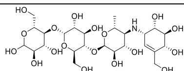
acarbose
