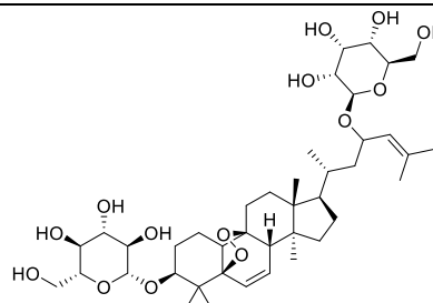
Goyaglycoside-f
