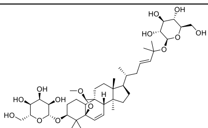
Goyaglycoside-g
