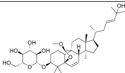
Goyaglycoside-a
