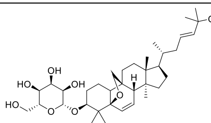
Momordicoside G
