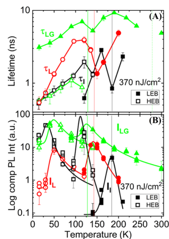
Figure 4. (a) Lifetime as a function of temperature for 352 nm-CL ( \tau_{LG} ), 550 nm-CS ( \tau_I ), and 103 nm-IS ( \tau_L ). Closed symbols correspond to the data of the LEB and the open symbols to the HEB. (b) Time-integrated PL intensity as a function of temperature for 352 nm-CL ( I_{LG} ), 550 nm-CS ( I_L ), and 103 nm-IS ( I_I ). Closed symbols correspond to the data of the LEB and the open symbols to the HEB.
