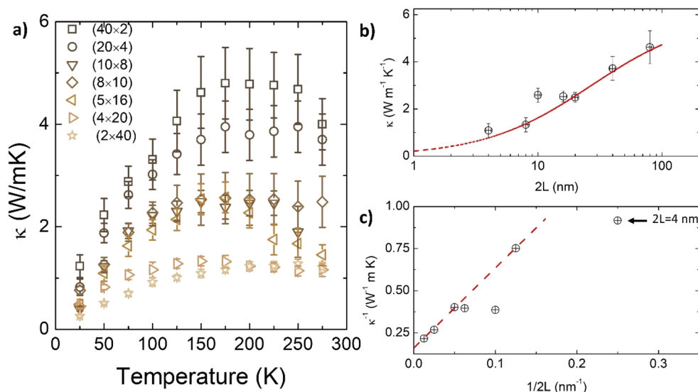
Figure 2. (a) Temperature dependence of the thermal conductivity of the different SLs with t = 80 nm (see Table S1 in the Supporting Information for further details of the periodicity of each sample). (b) Dependence of the thermal conductivity of the SLs at 150 K with the period 2L and the fitting to eq 1. (c) Linearized version of eq 1 and linear fitting of the experimental data. As discussed in the text, the validity of eq 1 at low values of L is compromised, when the Kaptiza and the period lengths, become comparable. For that reason, the data at 2L = 4 (marked with an arrow), was excluded from the fitting.
