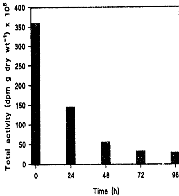
Fig. 1. Depletion of 14 C activity in the labelled coconut frond.
