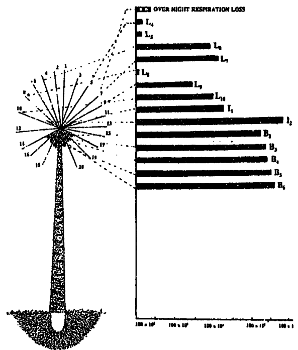
Fig. 3. Distribution of total 14 C activity (DPM) 7 days after labelling.
