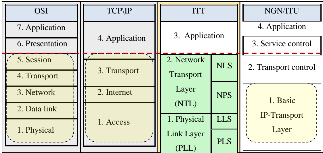
Figure 2 – The ITT open system interconnection model
