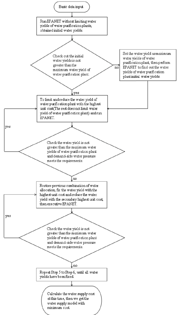
Fig. 1 Flowchart of the heuristic method
