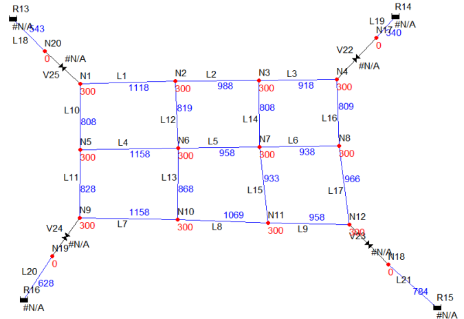
Fig. 3 System layout
