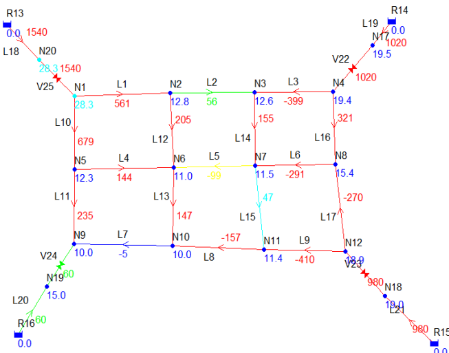
Fig. 5 Map of the hydraulic network analyzed using the exhaustive method.
