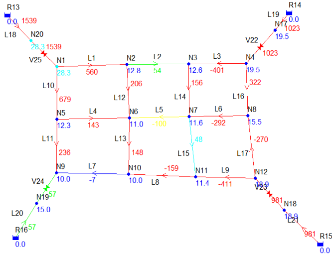
Fig. 4 Map of the hydraulic network analyzed using the heuristic method.
