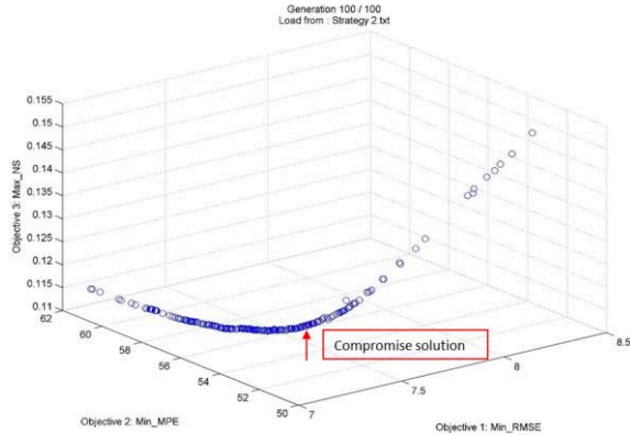
Fig. 5 Compromise solution in Pareto front of original case
