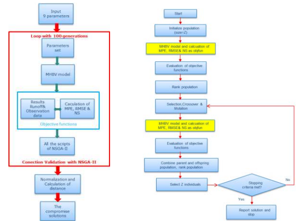
Fig. 3 Flowchart of linking MHBV model and NSGA-II algorithm
