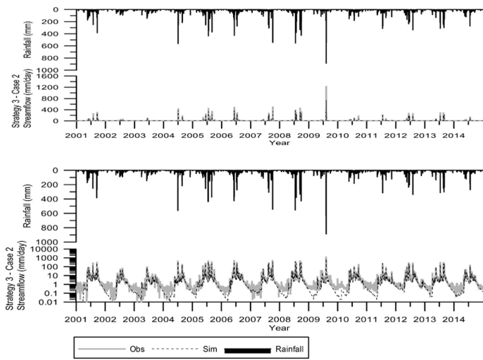
Fig. 7 Multi-objective function for simulated and observation hydrographs in validation period time (Strategy 3 – Case 2)
