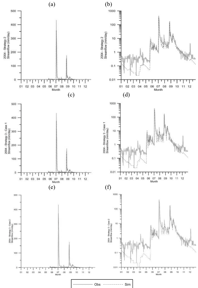
Fig. 8 The best case of simulation in validation period (2004). (a) and (b) are monthly streamflow simulation in Strategy 2, (c) and (d) are monthly streamflow simulation in Strategy 3 – Case 1, (e) and (f) are monthly streamflow simulation in Strategy – Case 2.
