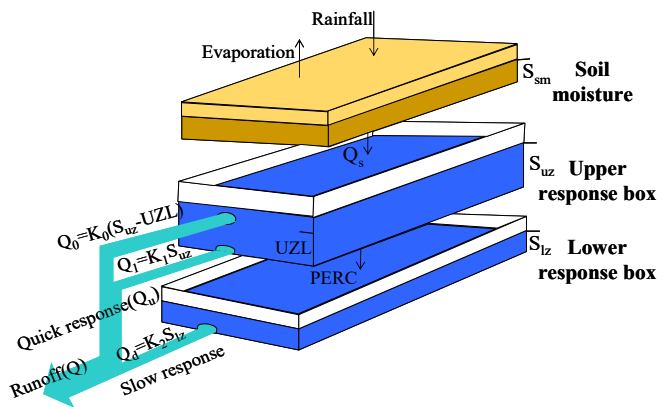
Fig. 2. Runoff responses, conceptual soil storage structure and water fluxes considered by the continuous rainfall-runoff model modified from HBV of Bergström (1976, 1992), which is referred to as MHBV
