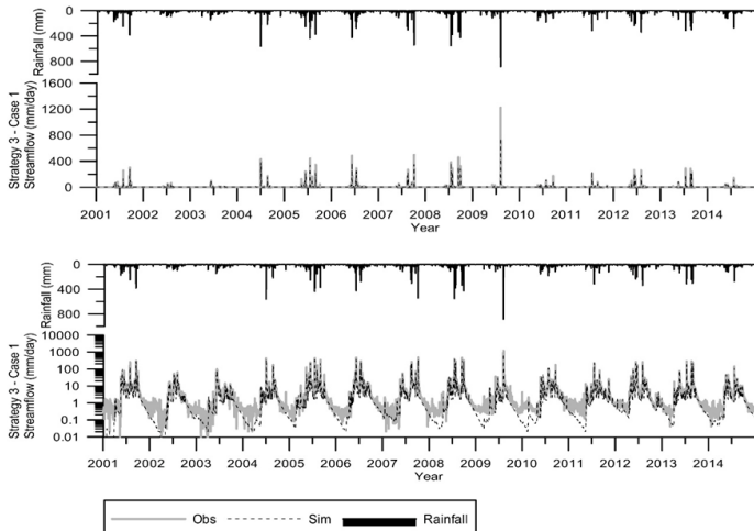
Fig. 6 Multi-objective function for simulated and observation hydrographs in validation period time (Strategy 3 – Case 1)
