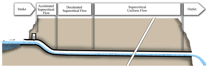
Fig. 2 SBT flow conditions sketch (adopted from Auel 2014).
