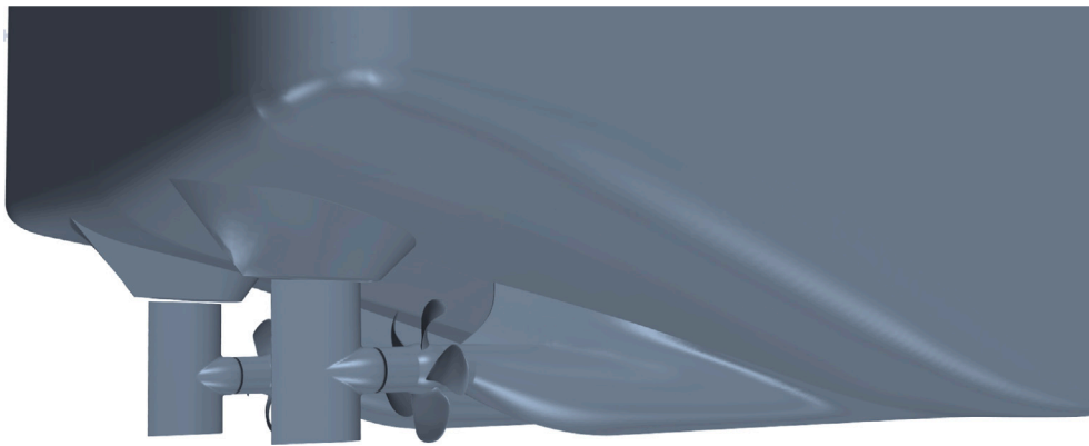
Fig. 2. Aft-ship geometry.
