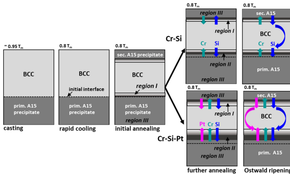
Fig. 10. Schematic of proposed coarsening mechanism showing the evolution of the precipitates from casting towards annealing. The different regions in the A15 phase and the \text{Cr}_{\text{ss}} /A15 interface are marked (I, II, III). Detailed explanations can be found in the text. Depending on the precipitates (primary or secondary) the diffusing species are shown.
