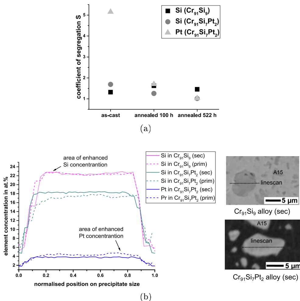
Fig. 5. (a) Segregation coefficient S of Si and Pt in Cr ss over annealing time. To demonstrate the tendency for segregation in the A15 phase, selected, normalised EPMA line scans measuring Si and Pt concentrations across A15 precipitates are shown in (b) for the binary and the ternary alloy after annealing for 522 h at 1200°C, respectively. For each composition a line scan across one primary (marked with prim ) and one secondary (marked with sec ) precipitate is shown. Corresponding BSE images of the investigated secondary precipitates are added.
