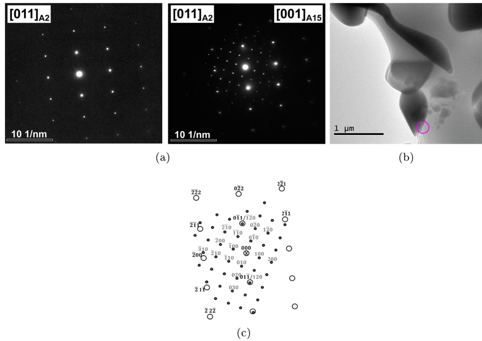
Fig. 6. SADPs of the \text{Cr}_{3\text{Si}} matrix (A2 structure) and the \text{Cr}_{3\text{Si}}/\text{A15} interface of the \text{Cr}_{91}\text{Si}_9 alloy after 100 h at 1200^\circ\text{C} annealing are shown in (a). In (b) the corresponding microstructure with the interface from which the SADP was taken (marked) and in (c) an indexed schematic of (a) are shown.
