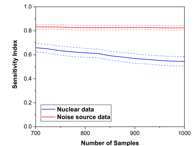
Fig. 14. The sensitivity indices of two groups with 95% confidence intervals varying with sample size (The straight line and the dashed line signify “mean value” and “95% confidence intervals”, respectively.).
